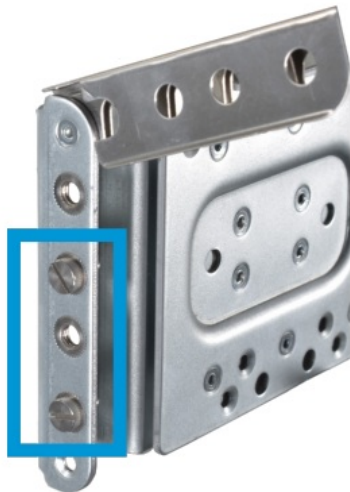
Round Hole Rack Pins
