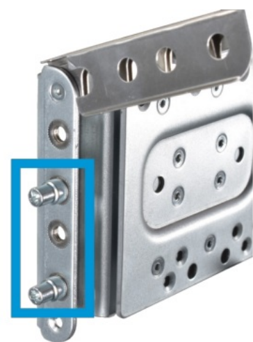
4mm Hole Rack Pins
