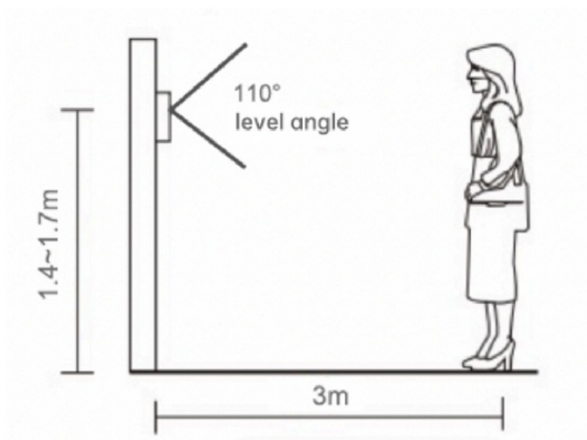
Image 1-1 Outdoor Station Installation Diagram
