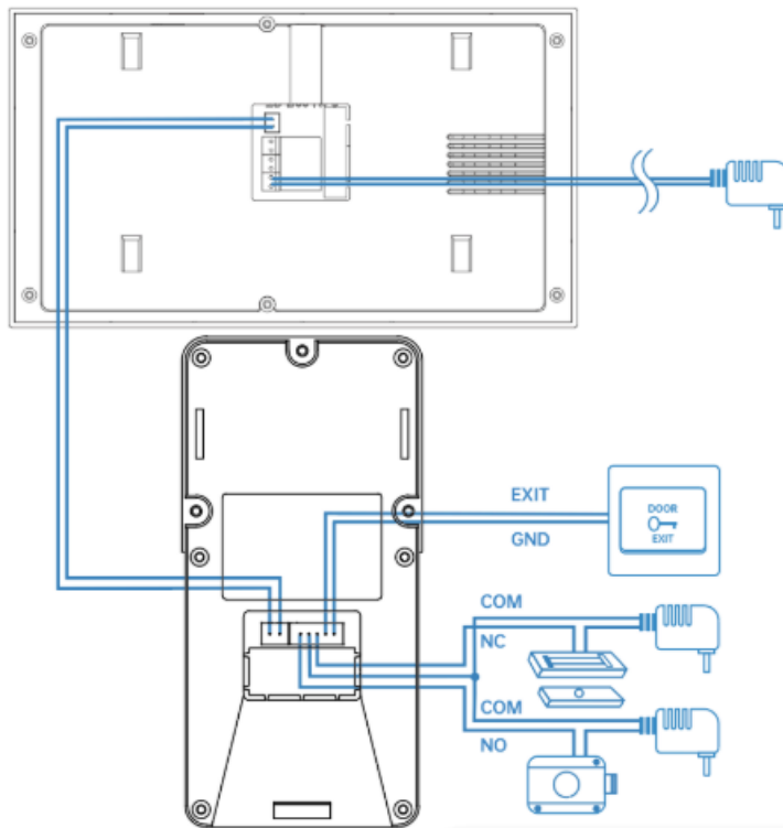
Image 1-3 1 Set Outdoor Station to 1 Set Indoor Monitor
