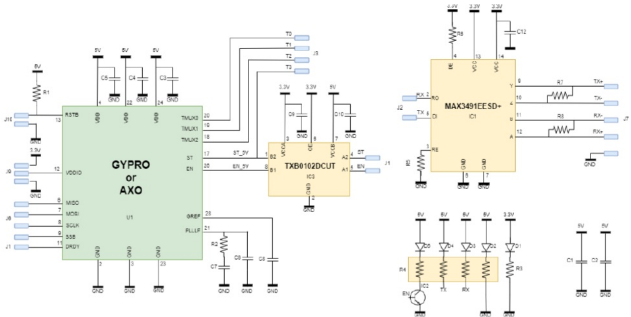
Figure 2: Electrical schematic
