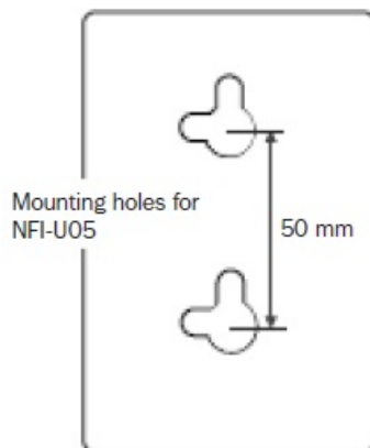
Mounting Holes for Drawing of NFI-U05
