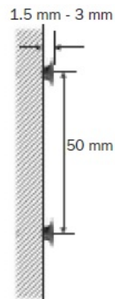
Screw Installation Distance
