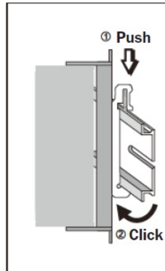
Removing the Switch
