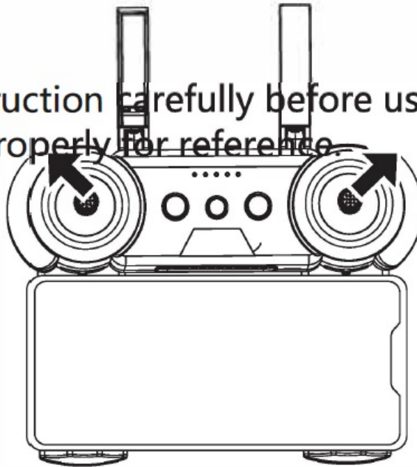
Geomagnetic calibration
