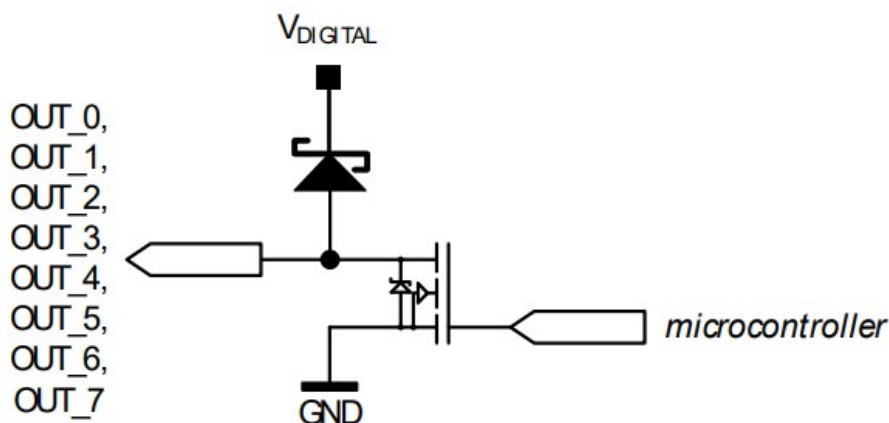
Figure 3.11 General purpose output (open-drain with freewheeling diode)
