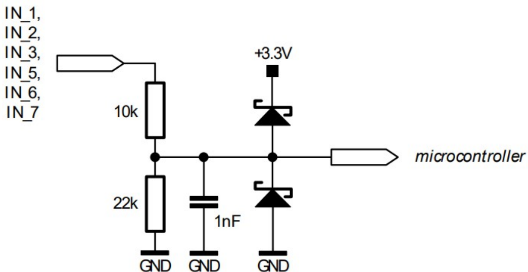
Figure 3.9 General purpose digital input circuit
