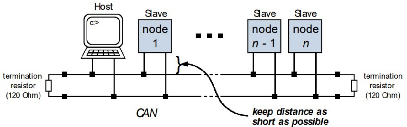
Figure 3.7 CAN bus structure
