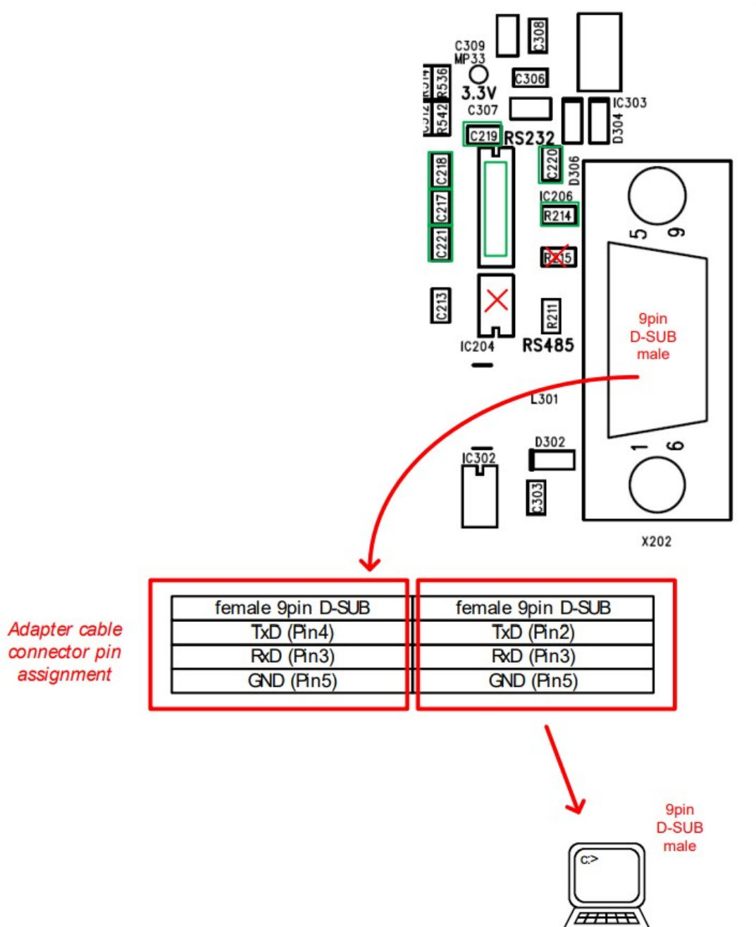
Figure 8.1: Using the RS232 assembly option instead of RS485
