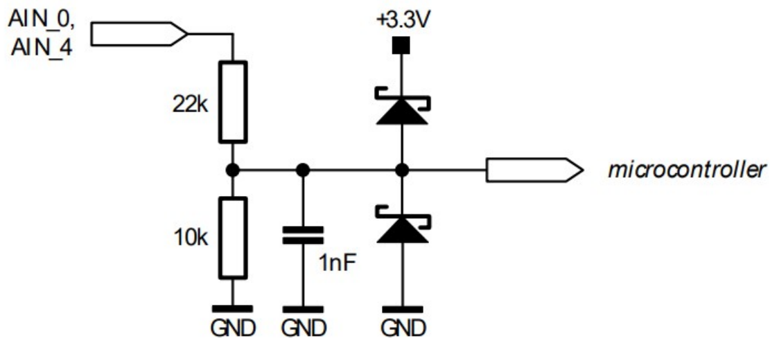
Figure 3.10 General purpose analog input circuit
