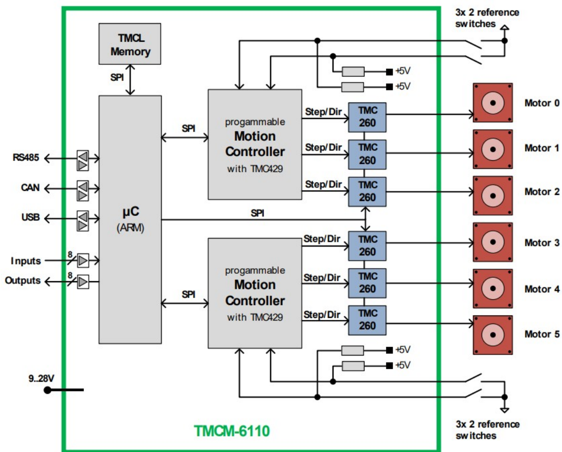
Figure 7.1: TMCM-6110 block diagram
