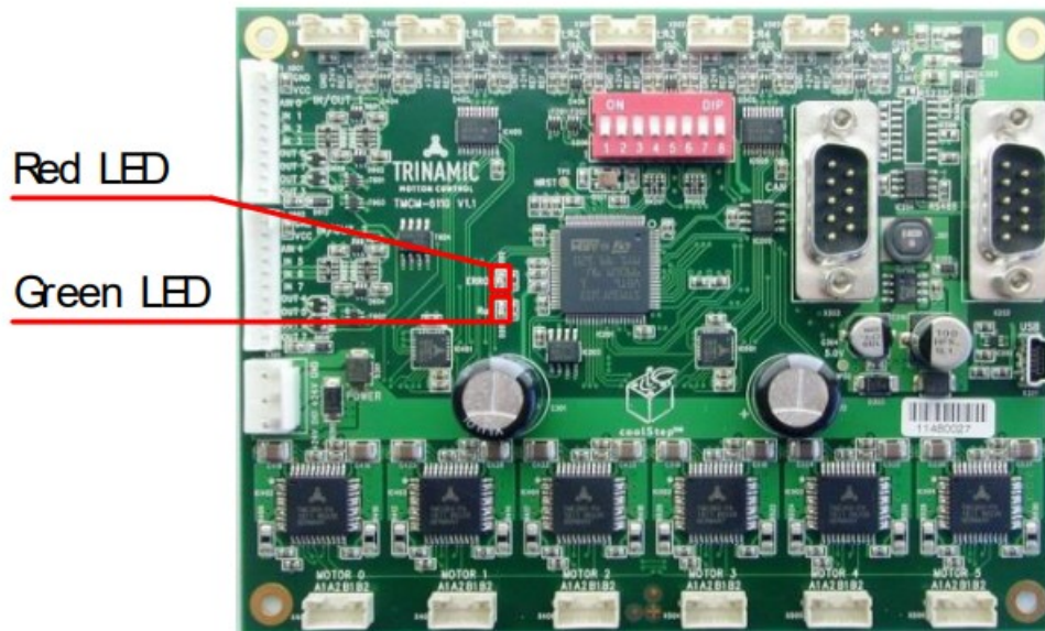
Figure 5.1 On-board LEDs
