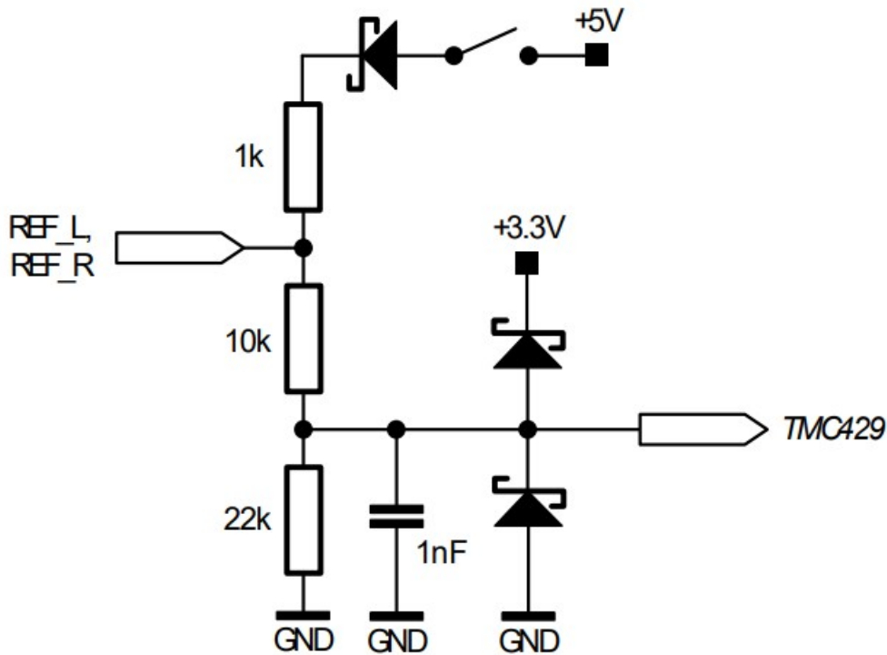
Figure 3.8 Reference switch input circuit (simplified diagram)
