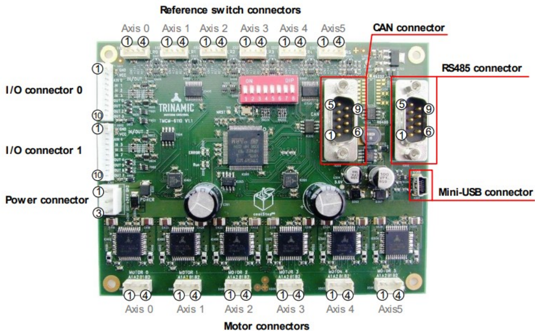
Figure 3.3 TMCM-6110 connectors
