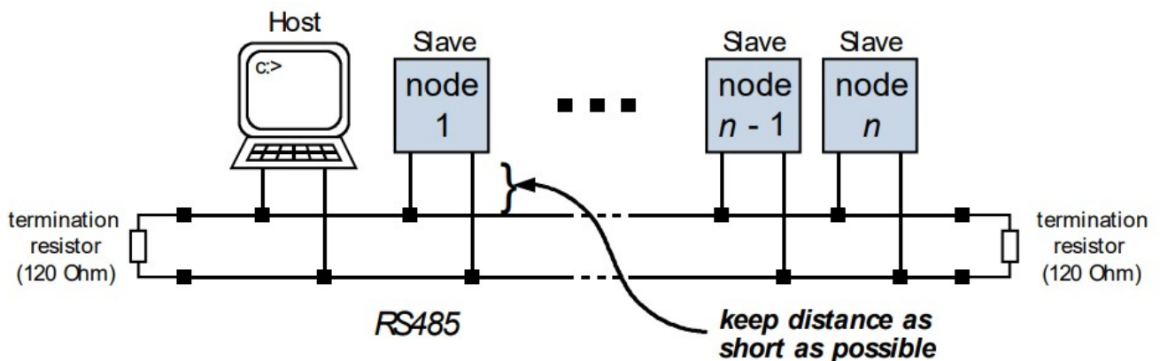
Figure 3.3: Bus structure
