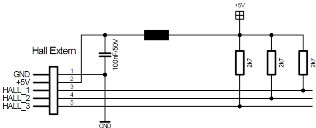
Figure 4.3: Hall sensor input circuit
