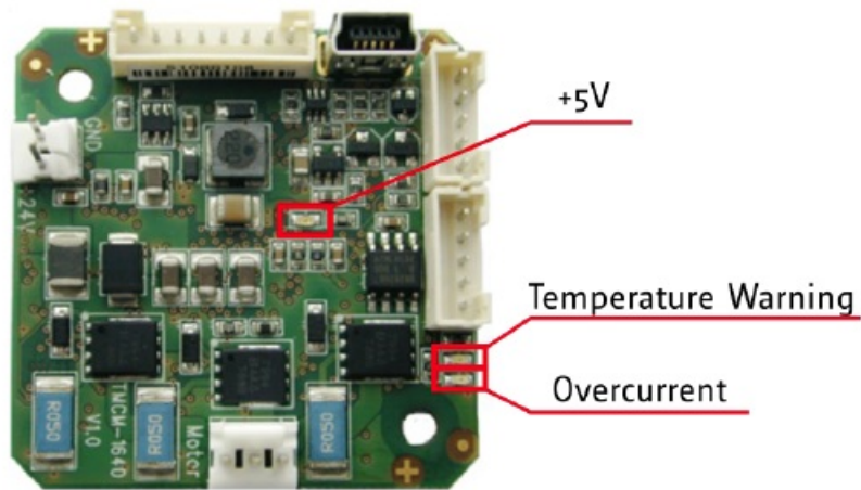
Figure 5.1 On-board LEDs
