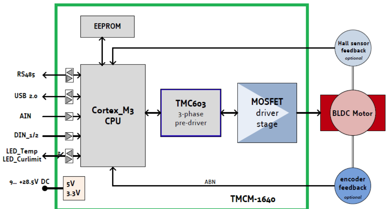
Figure 7.1: Main parts of the TCM-1640
