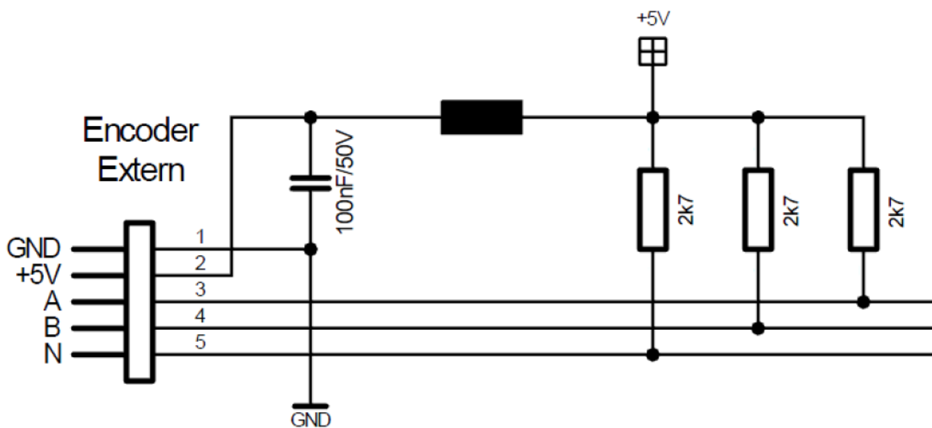
Figure 4.4: Encoder input circuit
