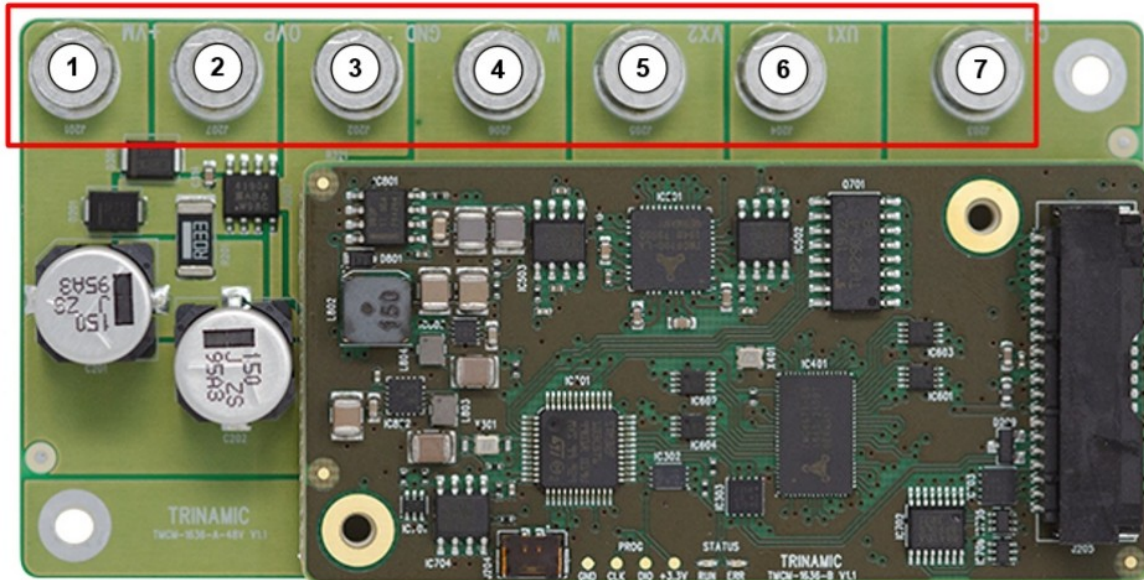
Figure 2: TMCN-1636 screw connectors
