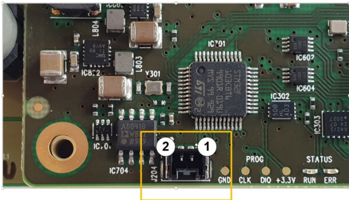
Figure 4: TCMC-1636 screw connectors
