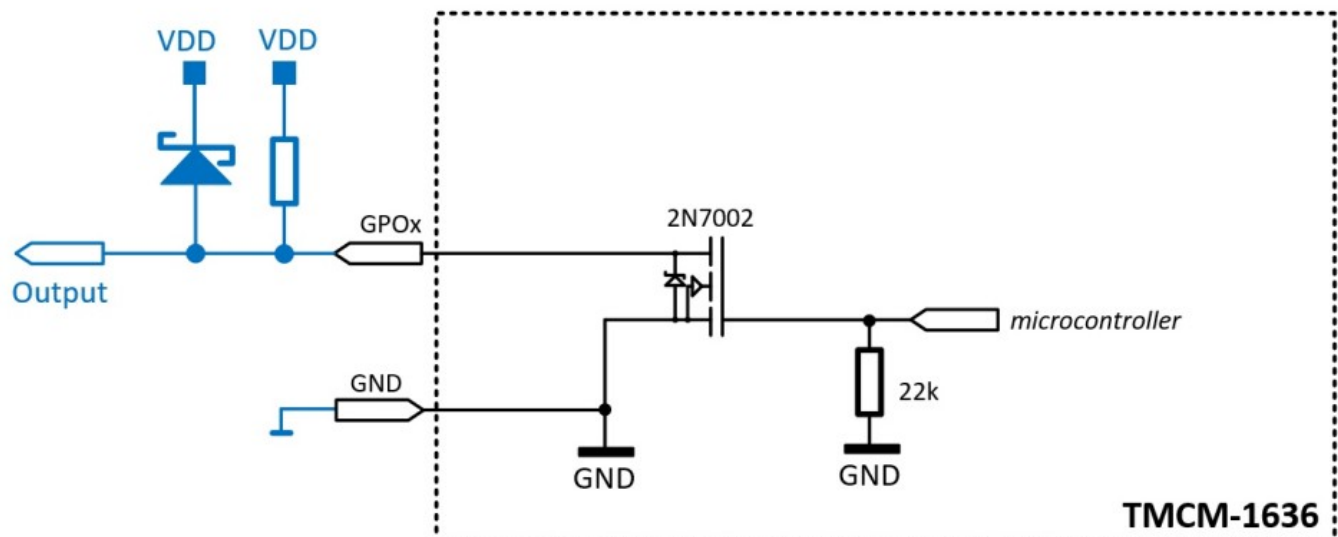
Figure 6: GPOx circuit
