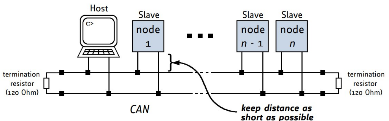
Figure 7: CAN bus structure with termination resistors
