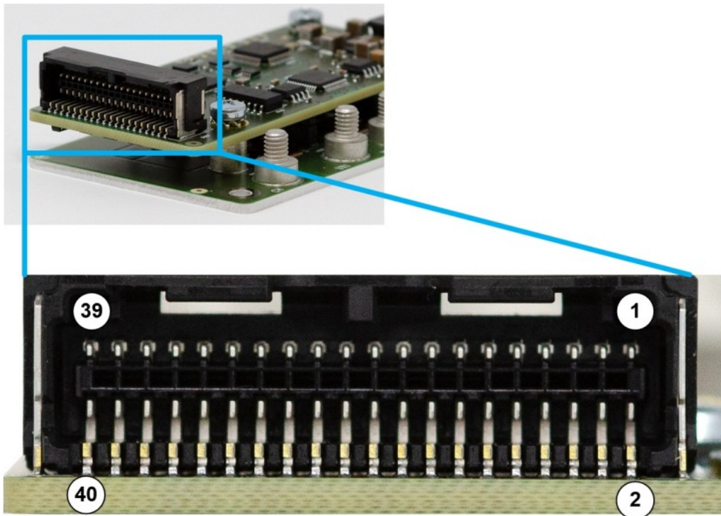
Figure 3: TCM-1636 I/O connector
