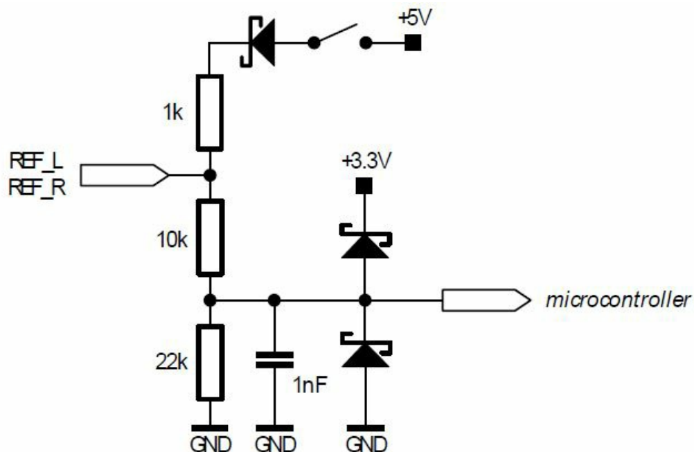
Figure 3.4 Reference switch input circuit (simplified diagram)
