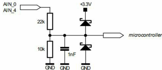
Figure 3.6 General purpose analog input circuit
