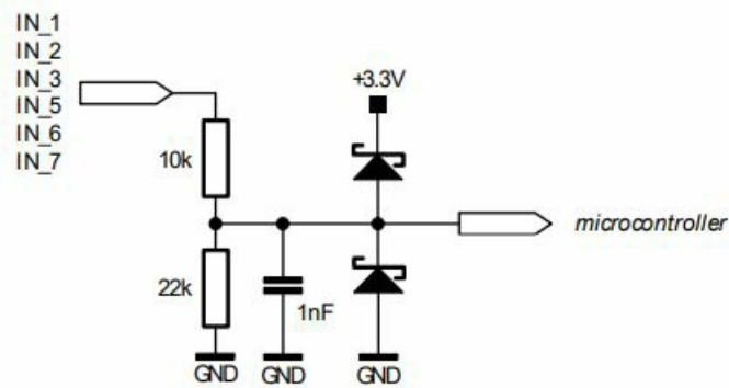
Figure 3.5 General purpose digital input circuit
