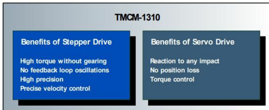
Figure 1.1 TMCM-1310 characteristics in closed loop mode
