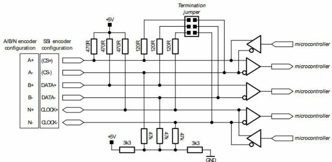
Figure 3.3 Encoder input circuit (simplified diagram)
