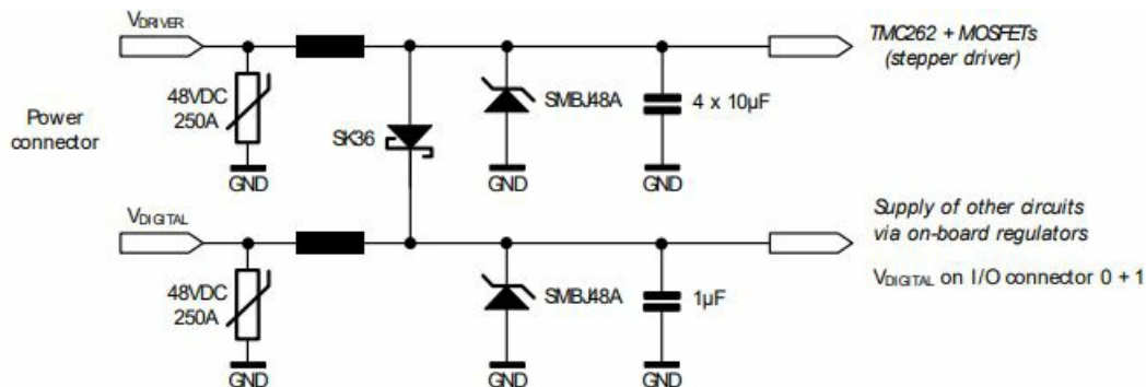
Figure 3.2 TCM-1310 power supply concept
