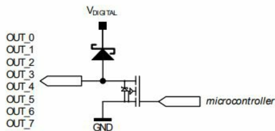
Figure 3.7 General purpose output (open-drain with freewheeling diode)
