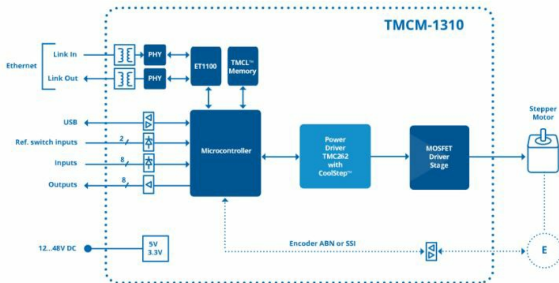
Figure 6.1 Main parts of TMC1310
