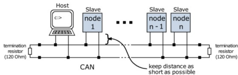
Figure 9: CAN bus structure
