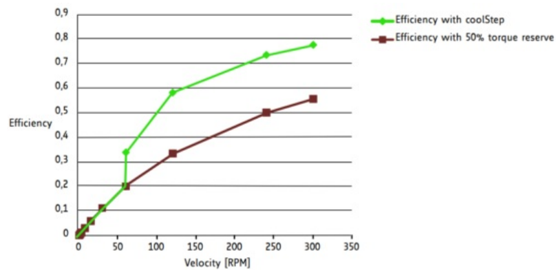
Figure 4: Energy Efficiency Example with coolStep
