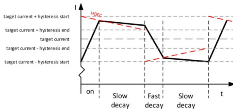
Figure 2: spreadCycle principle
