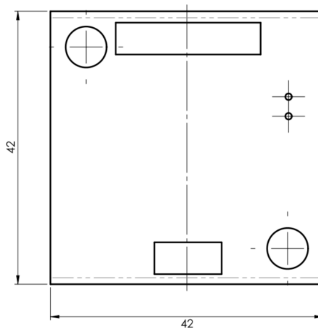
Figure 6: TMCM-1270 top view mechanical dimensions
