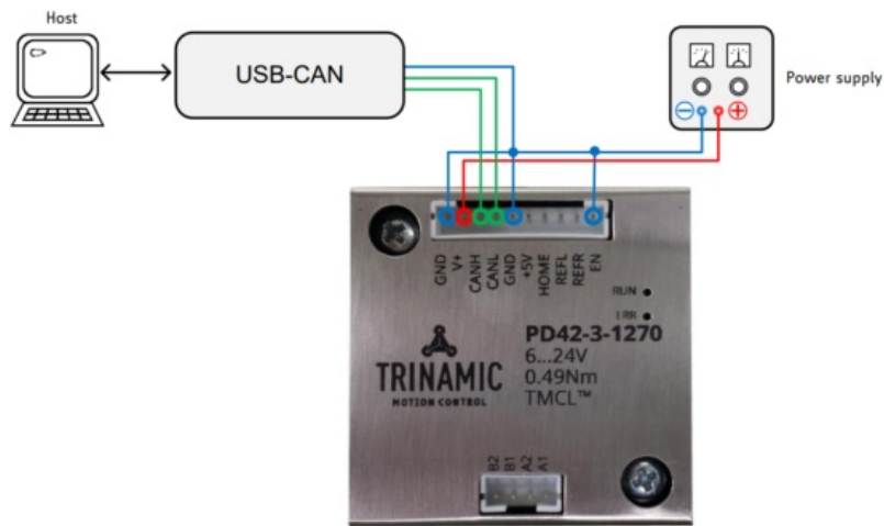
Figure 11: Typical application scenario for remote control of TMC-1270
