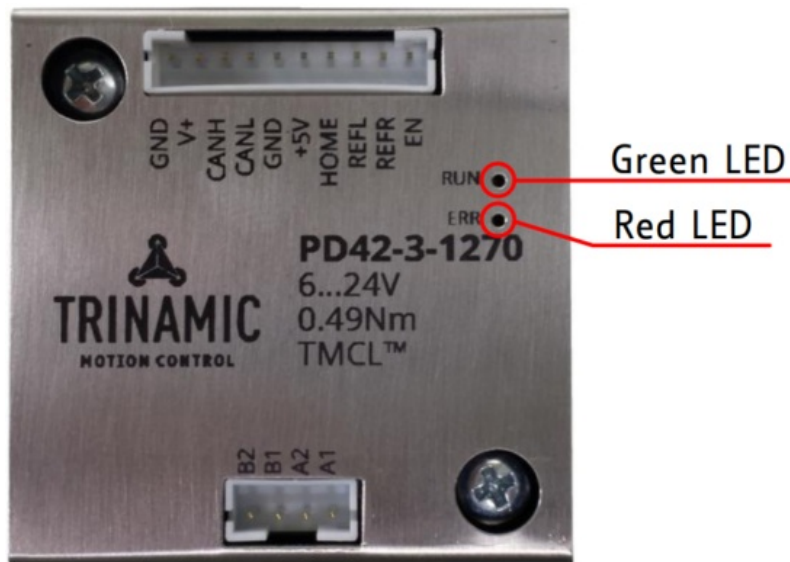
Figure 10: TMCM-1270 LED colors and loacation
