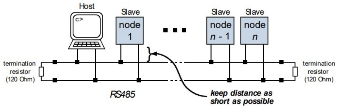
Figure 4.6: Bus structure
