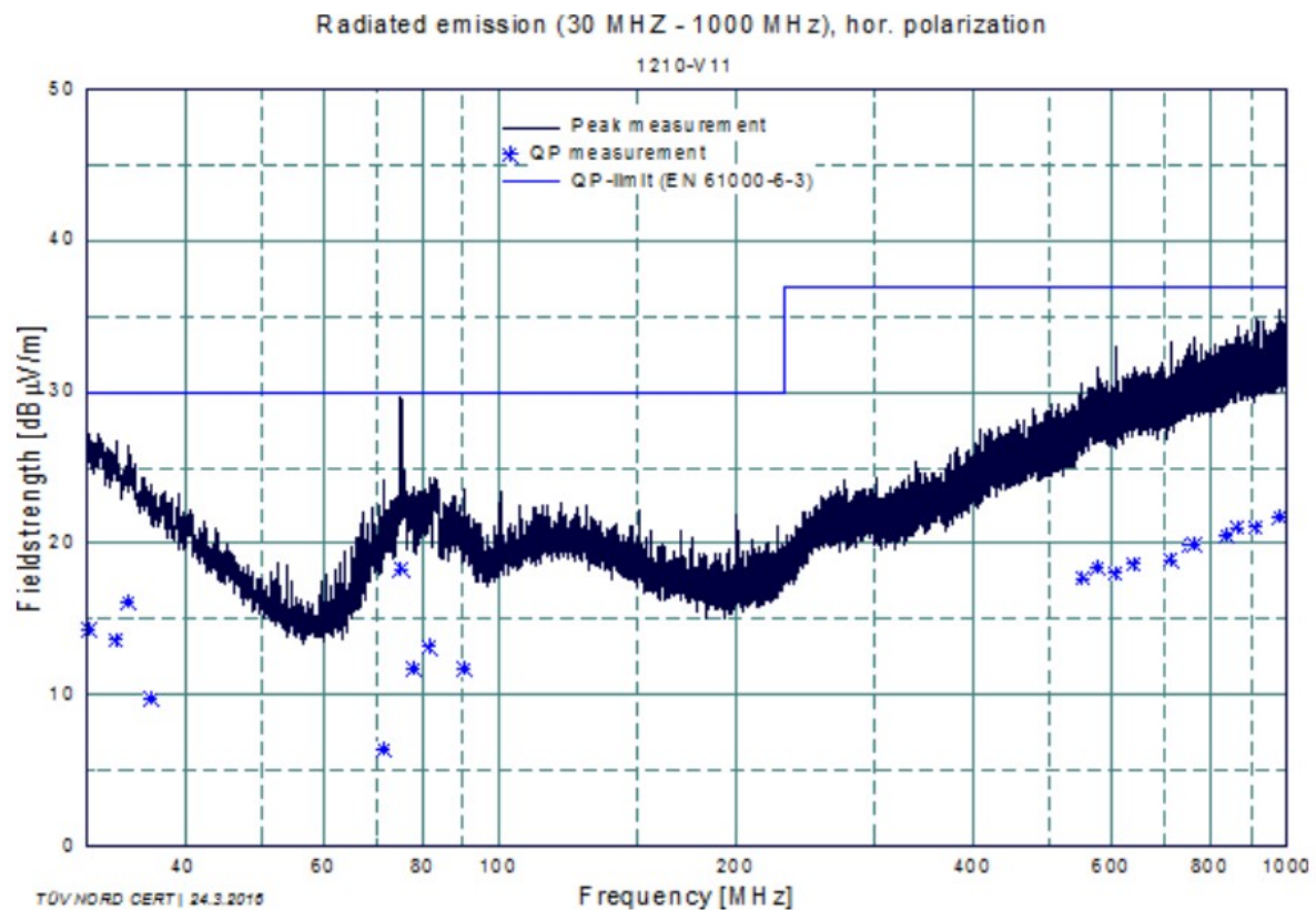
Figure 8.2: measurement results (example)
