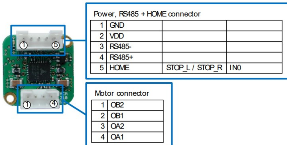
Figure 4.2 Overview connectors
