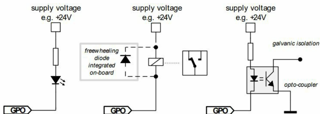
Figure 4.5 Possible circuits for GPO
