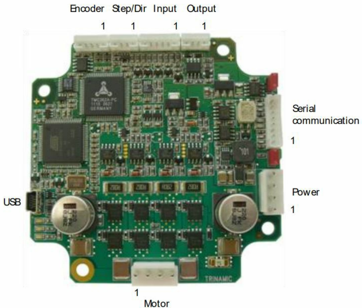
Figure 4.4 Overview connectors
