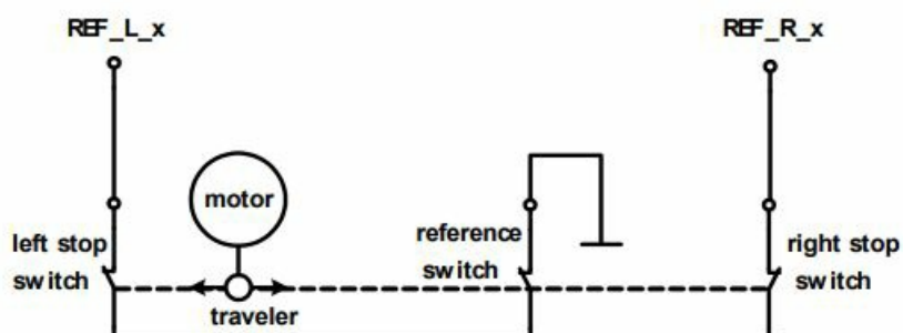
Figure 4.10 Limit switch and reference switch
