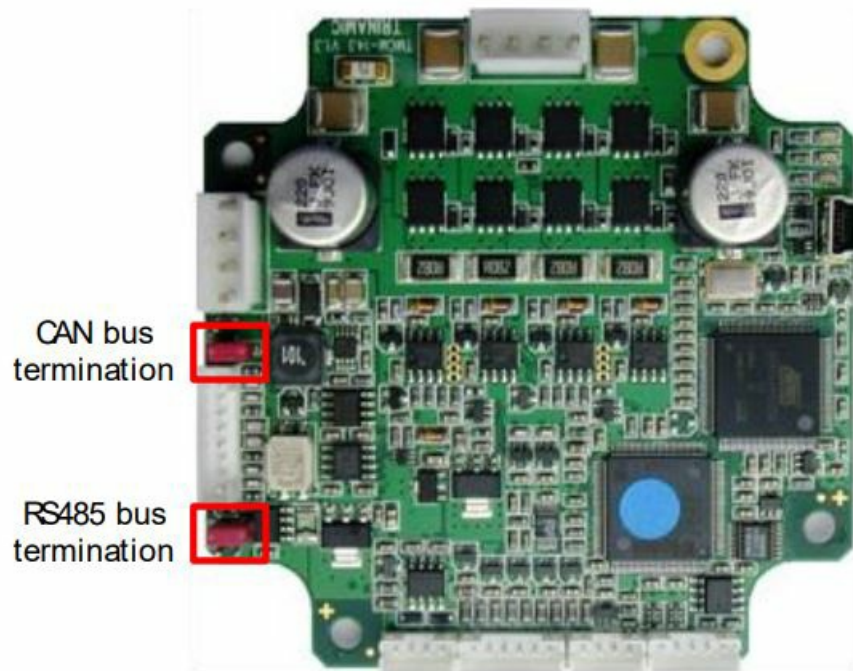
Figure 5.1 RS485 and CAN bus termination
