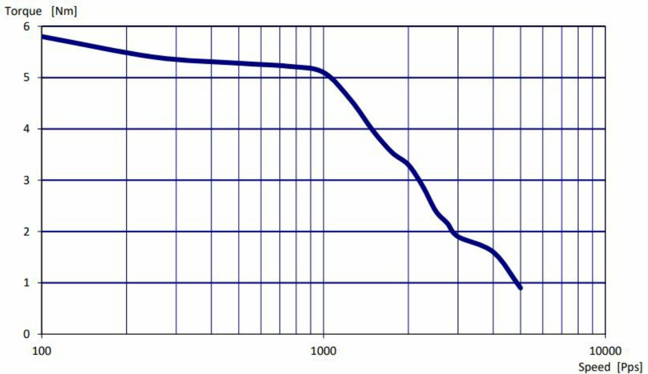
Figure 4.3 QSH8618-96-55-700 speed vs. torque characteristics
