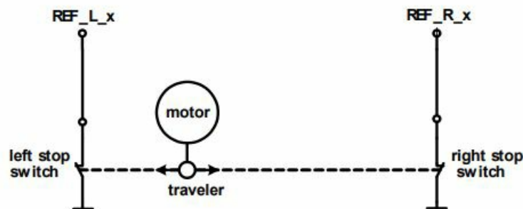
Figure 4.9 Left and right limit switches
