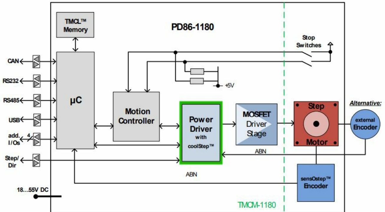
Figure 7.1 Main parts of the PD86-1180
