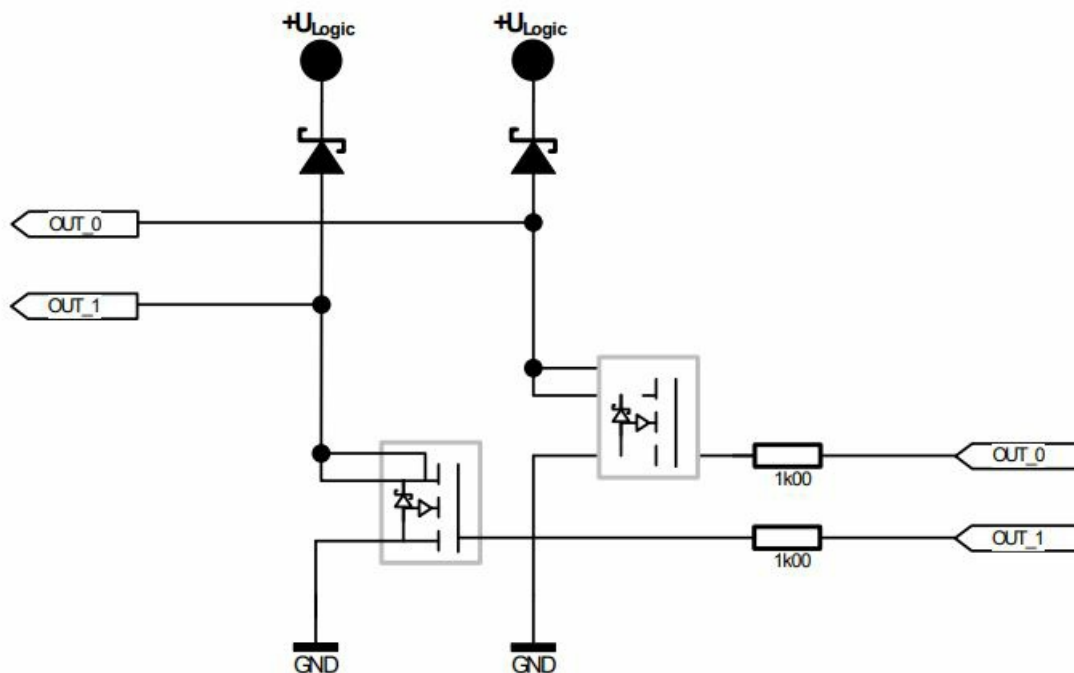
Figure 4.6 Internal circuit of the outputs
