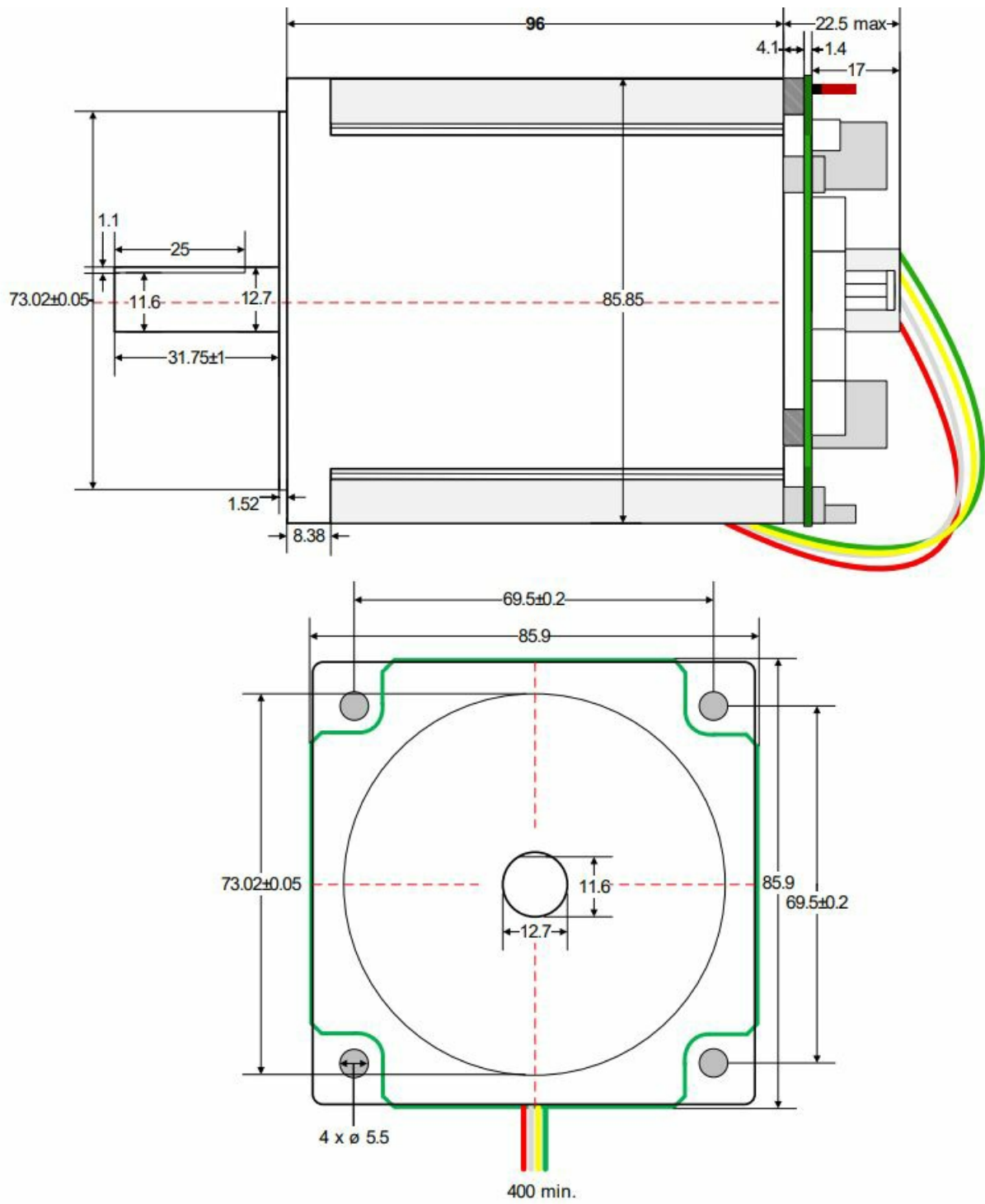
Figure 4.2 PD86-3-1180 dimensions
