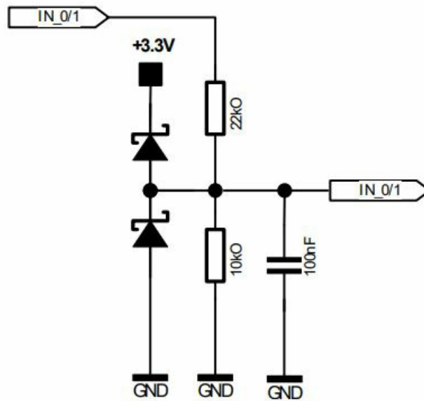
Figure 4.8 Internal circuit of the inputs
