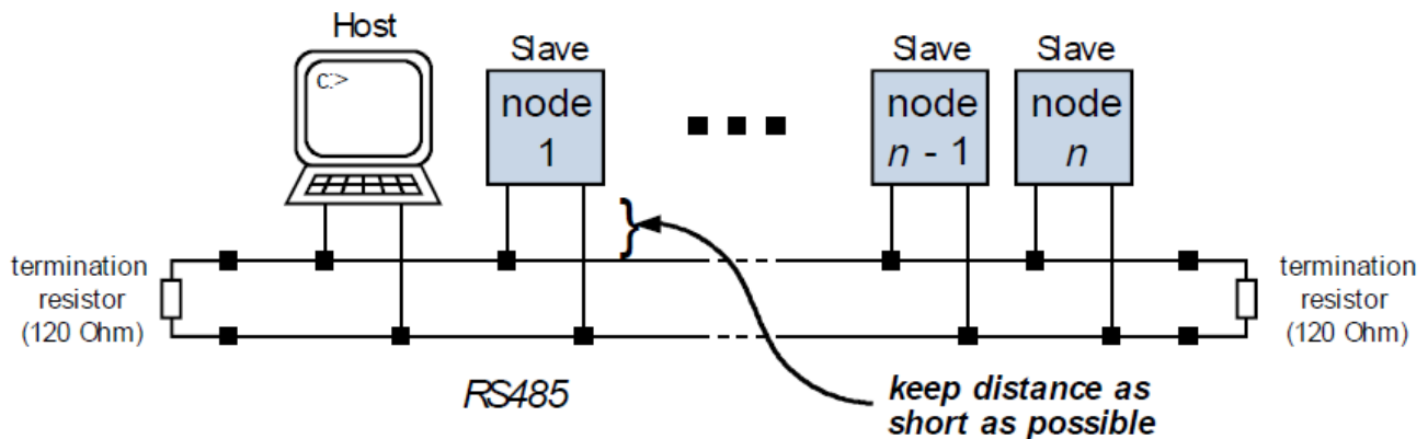
Figure 6.4 Bus structure
