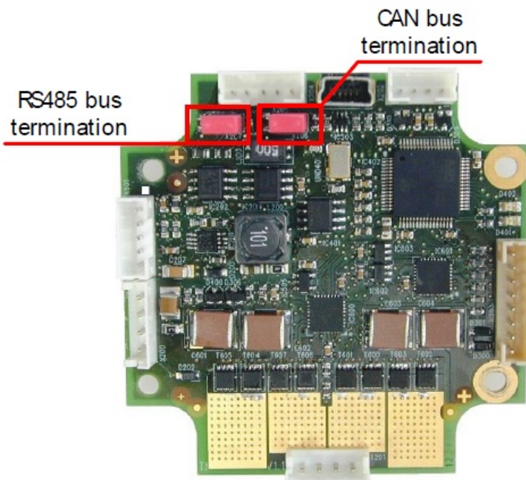
Figure 4.1 RS485 and CAN bus termination
