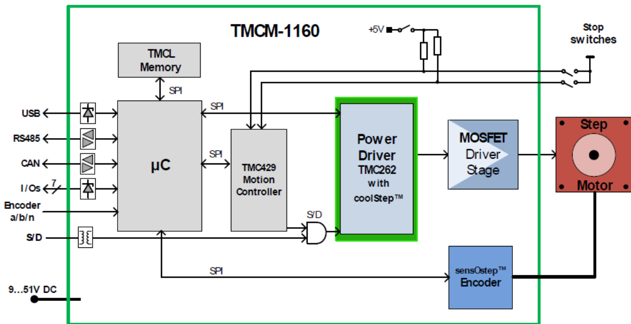
Figure 8.1 Main parts of the TMCM-1160
