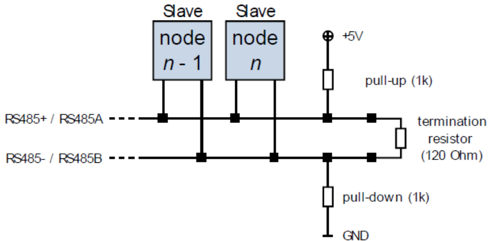
Figure 3.5 Bus lines with resistor network
