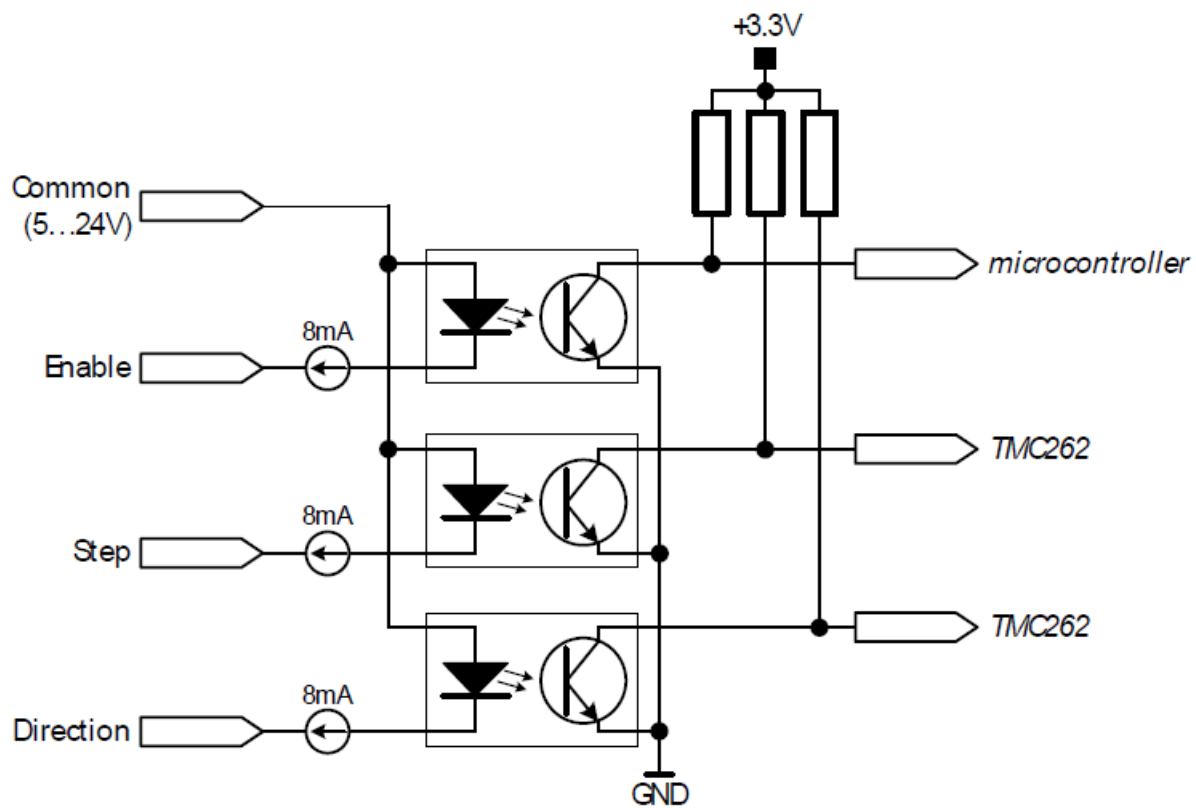
Figure 3.9 Step / Direction / Enable inputs
