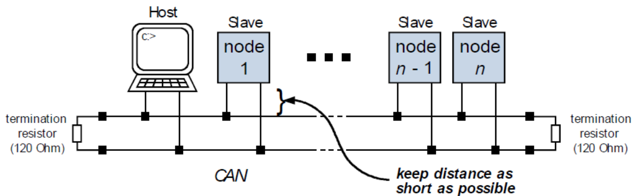
Figure 3.6 CAN bus structure
