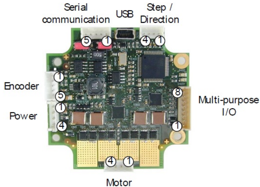
Figure 3.2 Overview connectors
