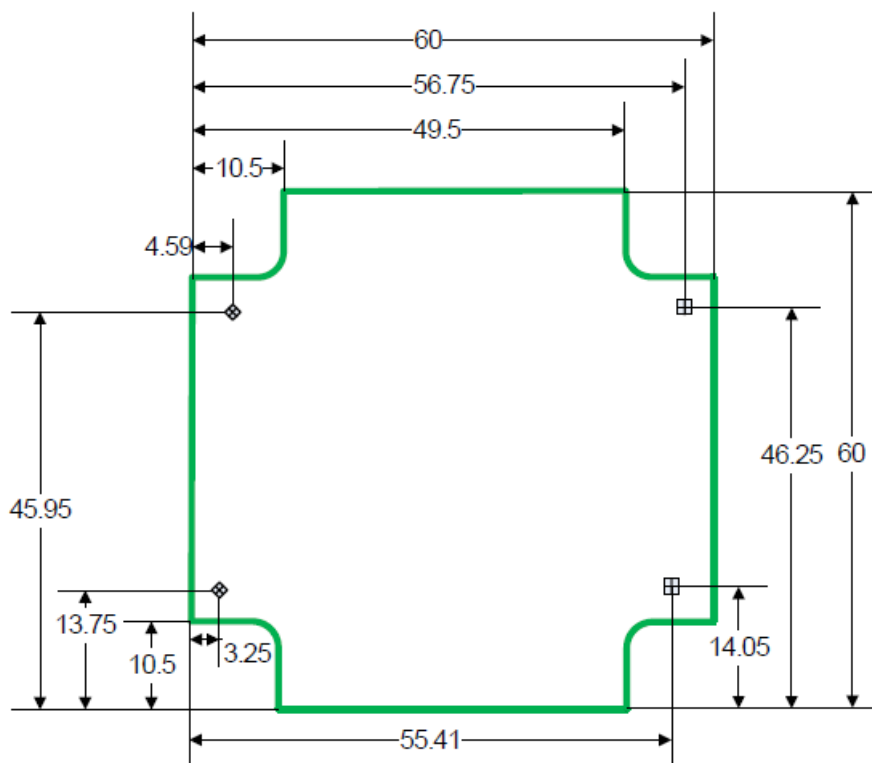
Figure 3.1 Dimensions and mounting holes
