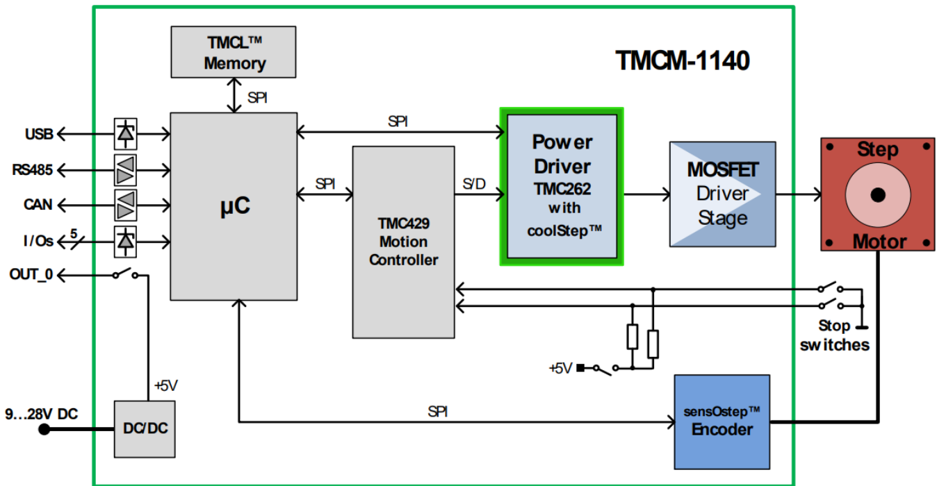
Figure 8.1 Main parts of the TCMCM-1140
