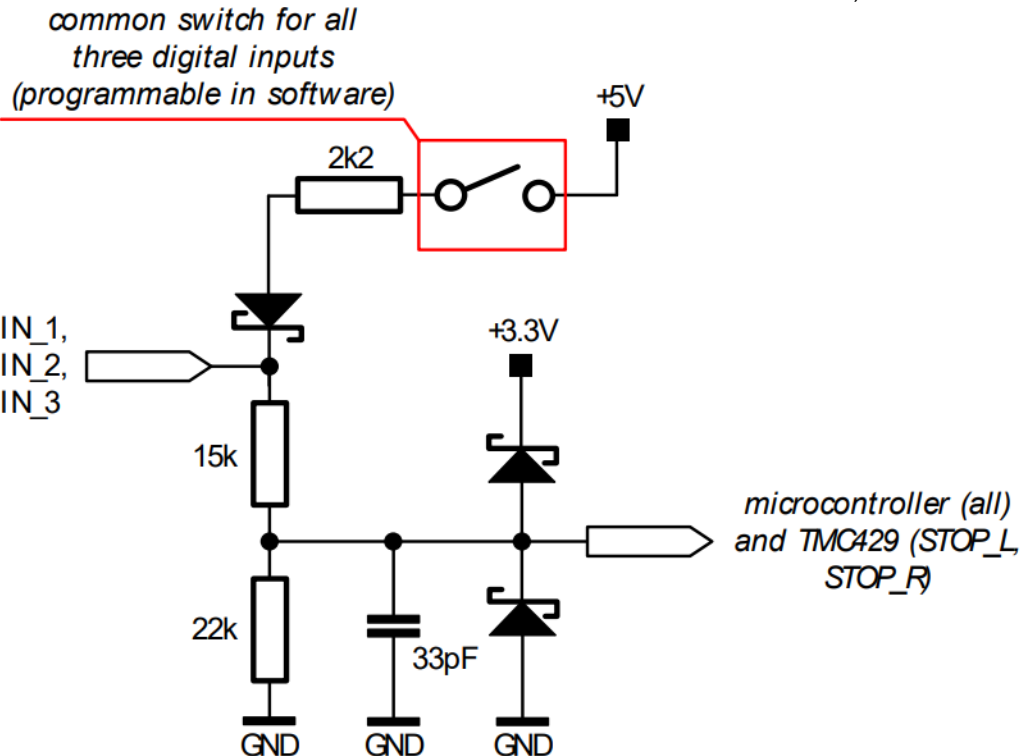
Figure 3.7 General purpose inputs (simplified input circuit)
