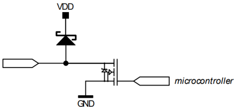
Figure 3.9 General purpose output OUT_0 (simplified circuit)
