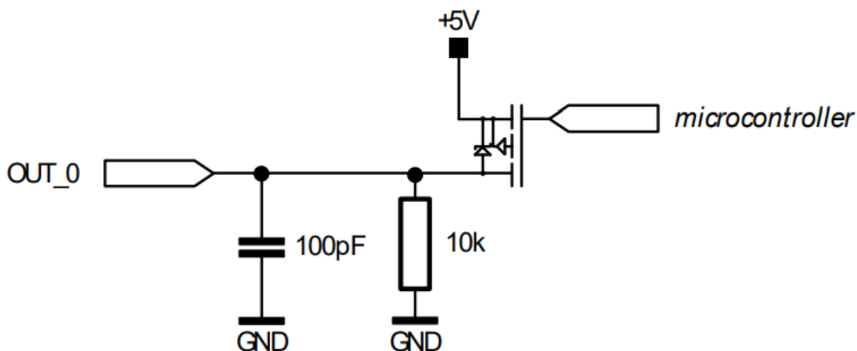
Figure 3.10 General purpose output OUT_1 (simplified circuit)
