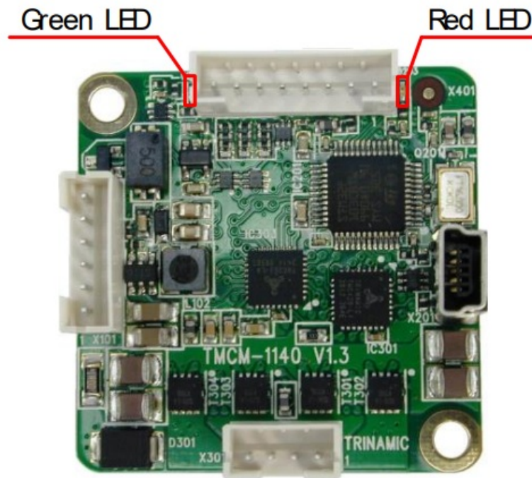
Figure 6.1 On-board LEDs
