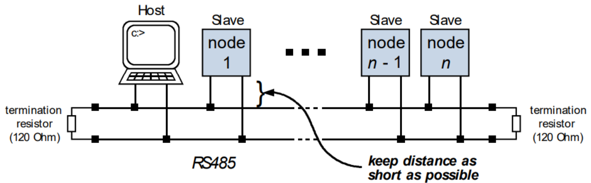
Figure 3.3: Bus structure
