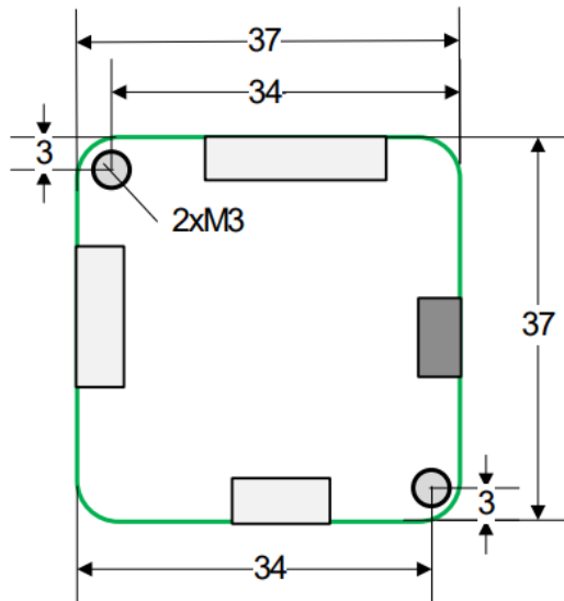
Figure 3.1 Dimensions of TCMC-1140 and position of mounting holes
