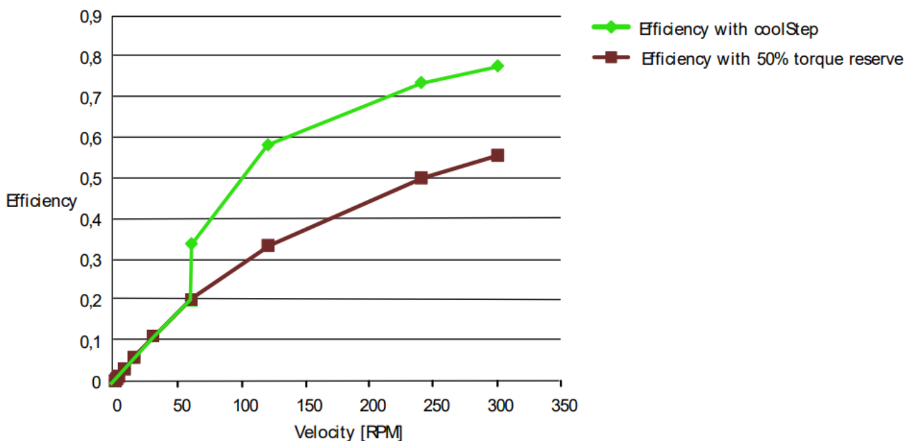
Figure 1.2 Energy efficiency example with coolStep
