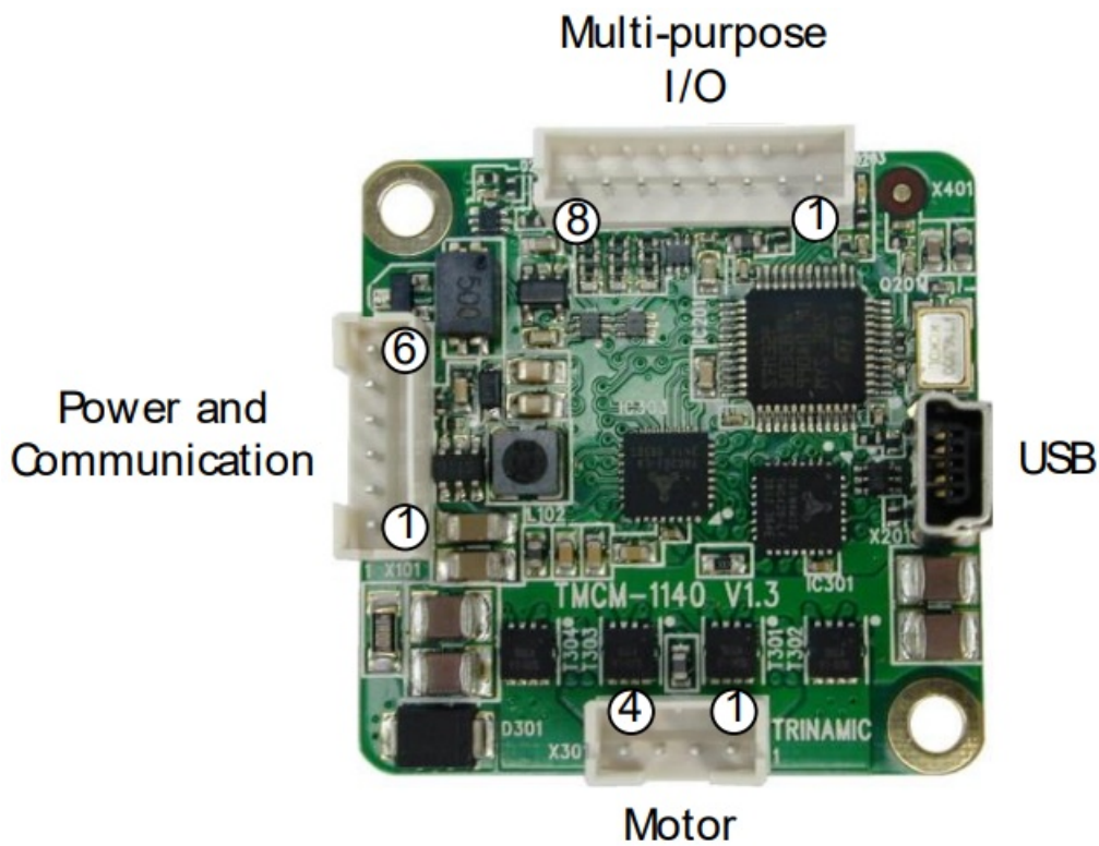
Figure 3.2 Overview connectors
