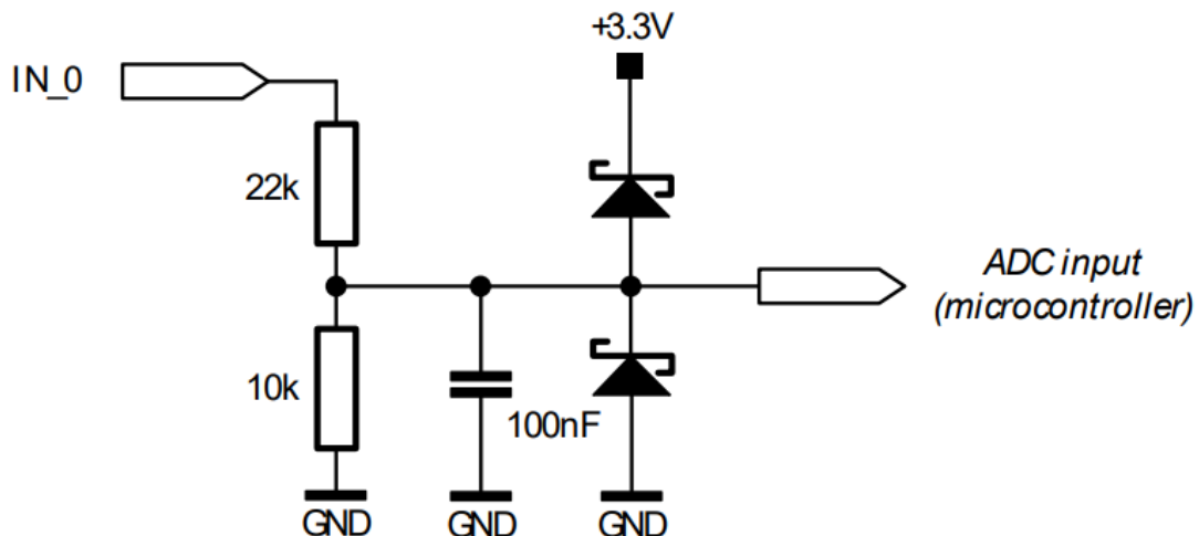
Figure 3.8 General purpose inputs (simplified input circuit)
