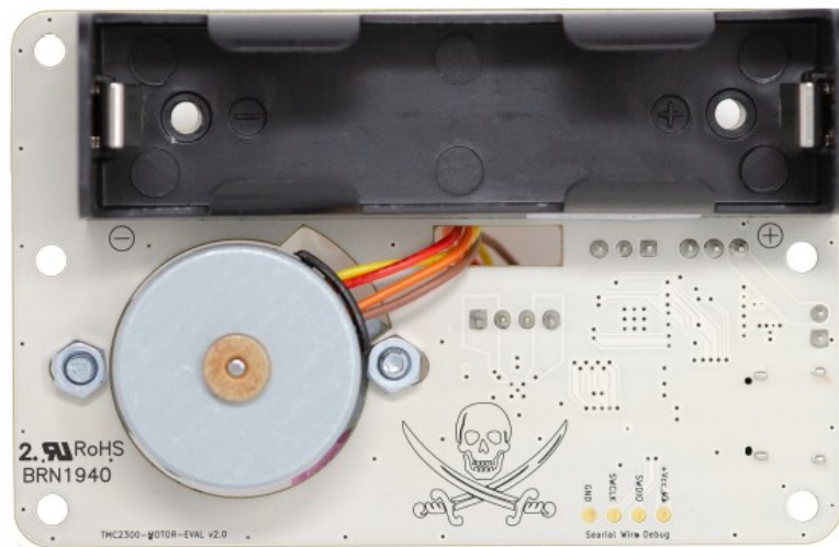
Figure 7: Battery holder on bottom side
