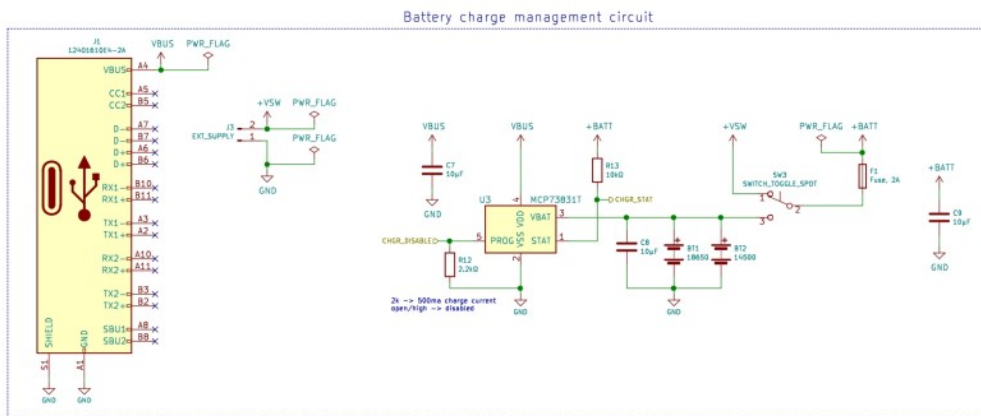
Figure 11: Battery charger circuit
