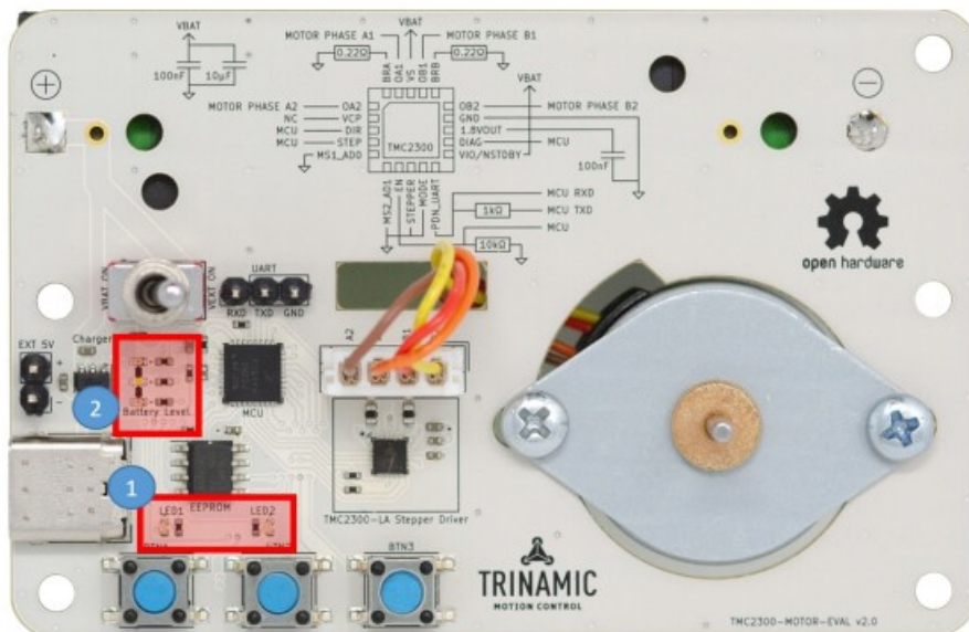
Figure 6: Top side LEDs
