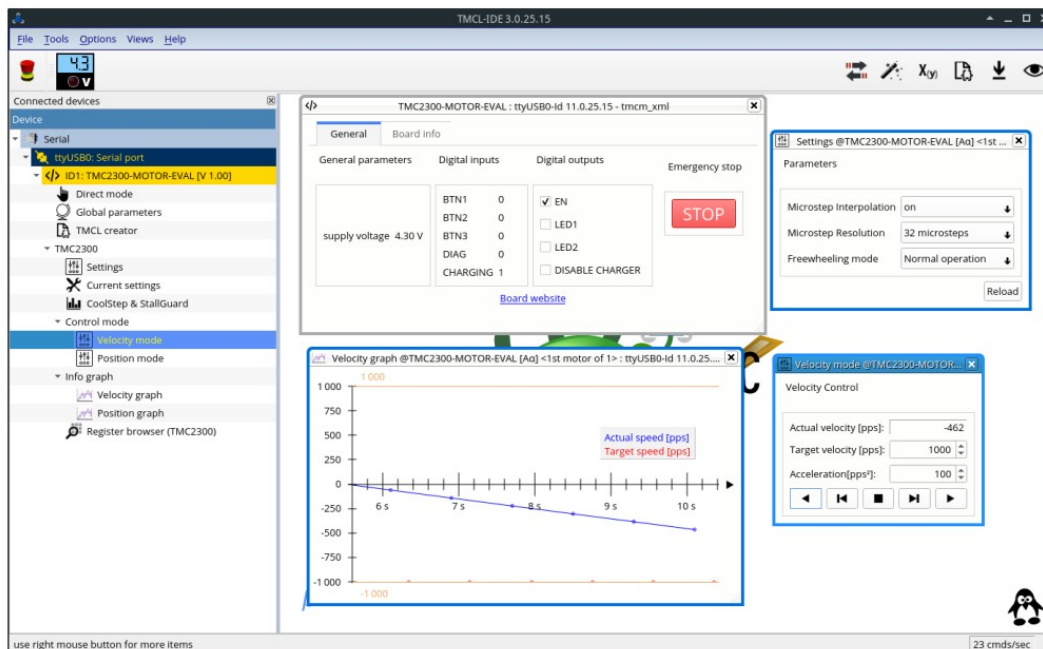
Figure 3: TMCL-IDE full view
