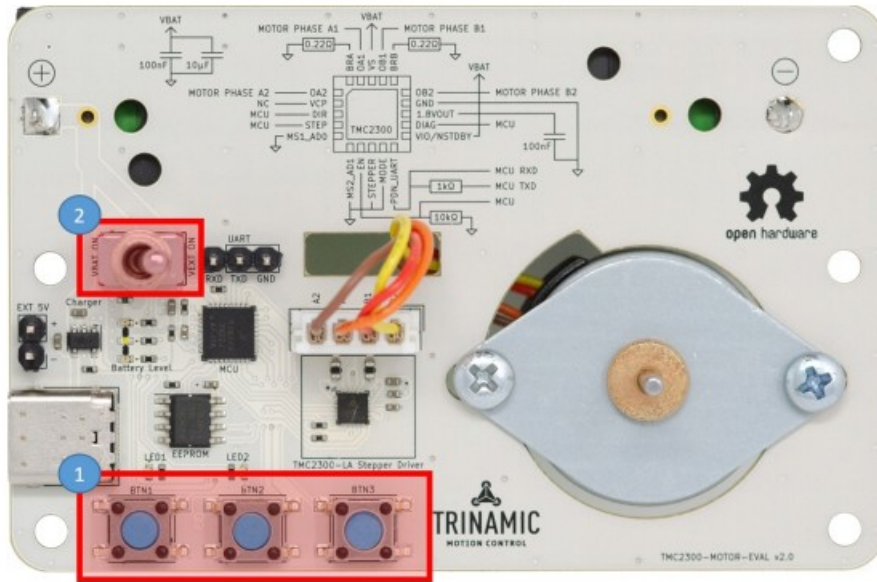
Figure 5: Top side Switches and Buttons
