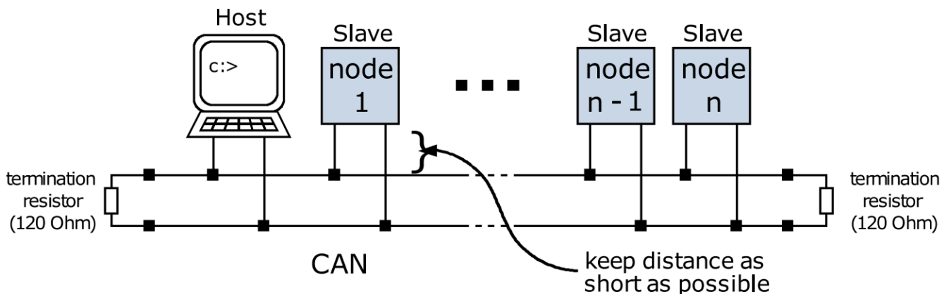
Figure 13: CAN bus structure
