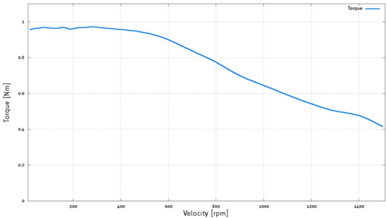
Figure 8: PD60-3-1378 torque vs. velocity 48V / 2.8A, 256 \mu steps
