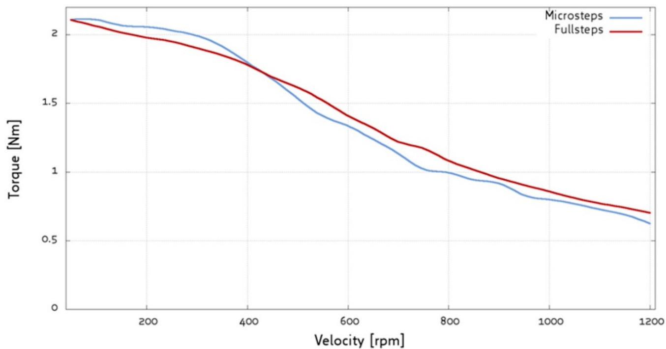
Figure 9: PD60-4-1378 torque vs. velocity 48V / 2.8A, 256μsteps
