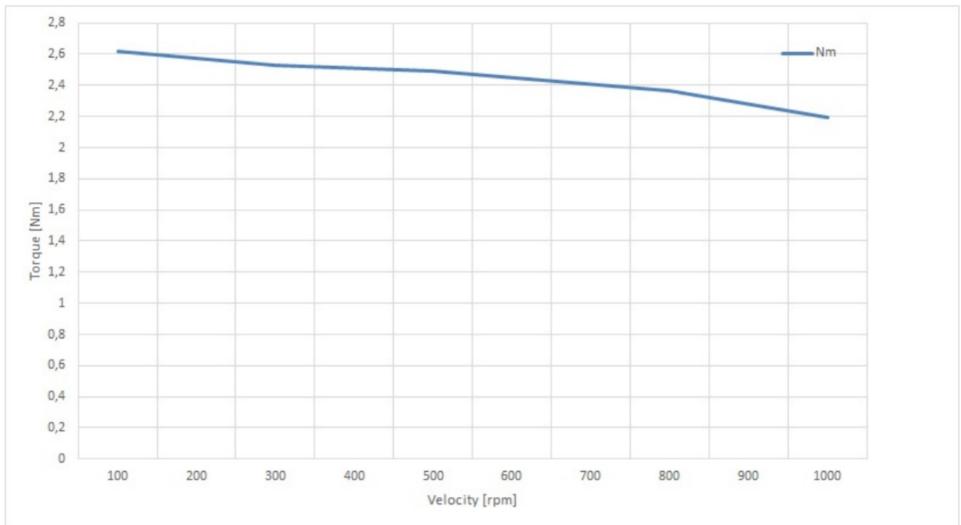
Figure 11: PD86-3-1378 torque vs. velocity 48V / 5.5A, 256μsteps
