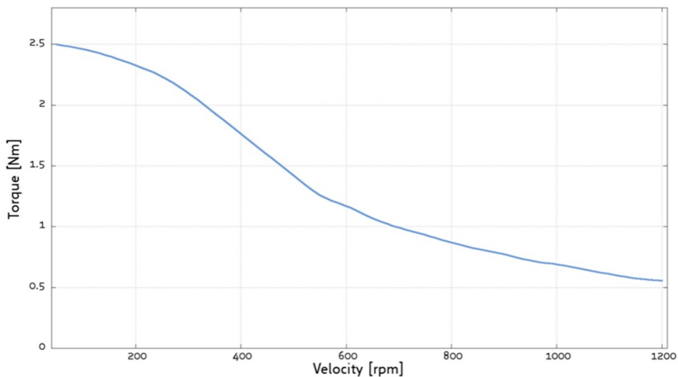
Figure 10: PD60-4H-1378 torque vs. velocity 48V / 9A, 256μsteps
