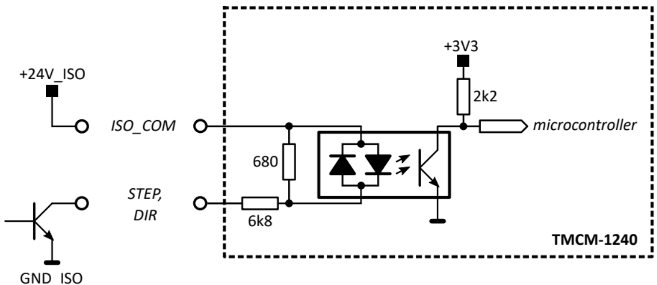
Figure 9: Step/Direction input
