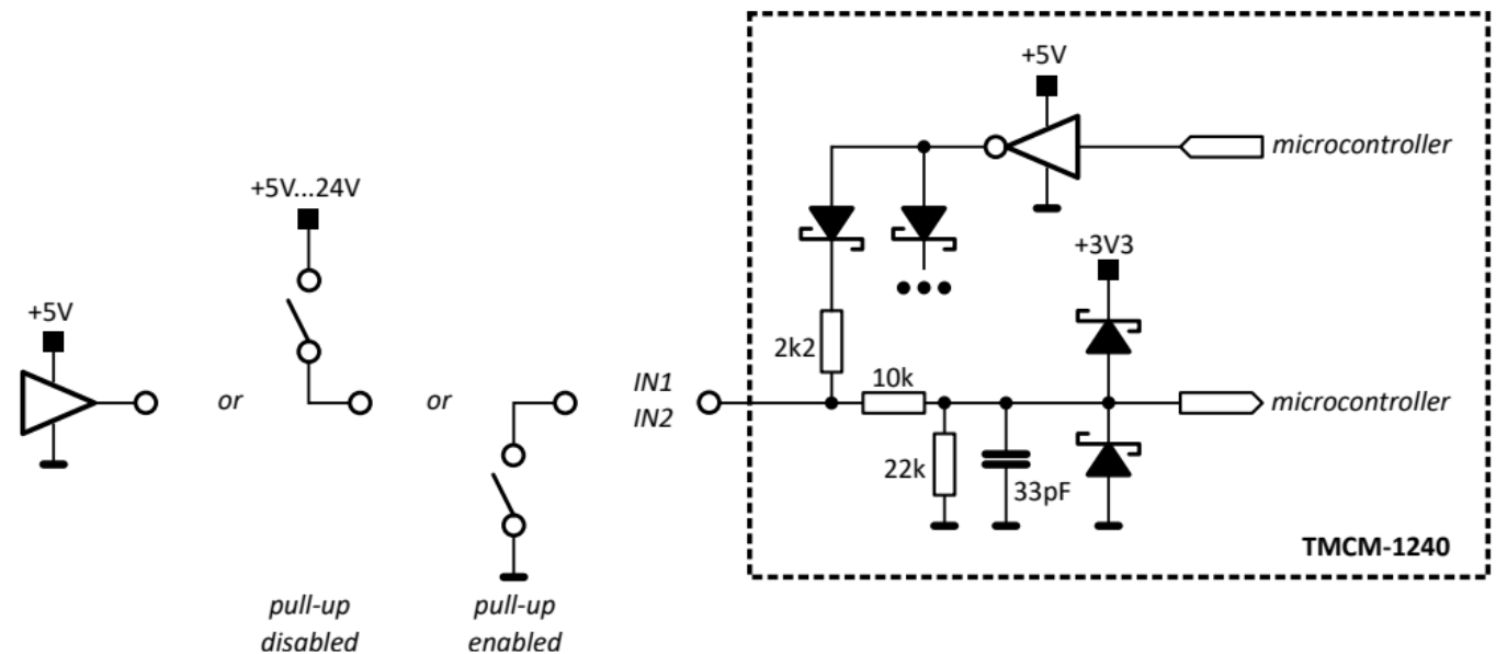
Figure 6: Digital inputs IN1 and IN2
