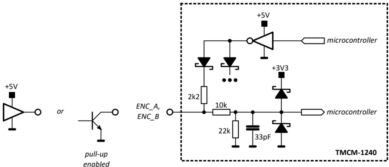
Figure 8: External encoder input
