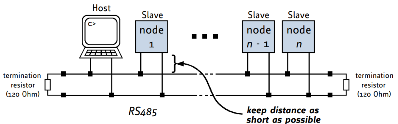
Figure 10: RS485 bus structure with termination resistors
