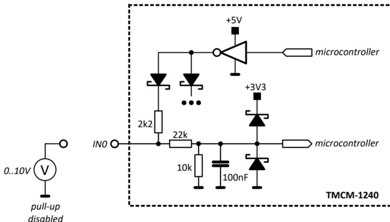
Figure 5: Analog input IN0
