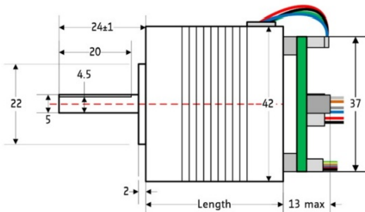
Figure 1: PD42-x-1240 with different NEMA17 / 42mm stepper motors (all dimensions in mm)
