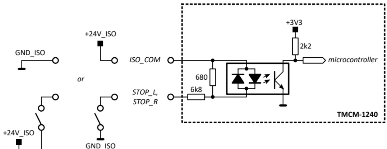
Figure 7: Stop switch inputs
