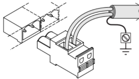
Push-fit terminal plug
