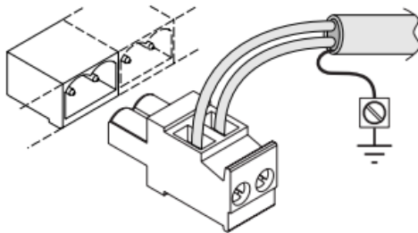
Screw terminal plug
