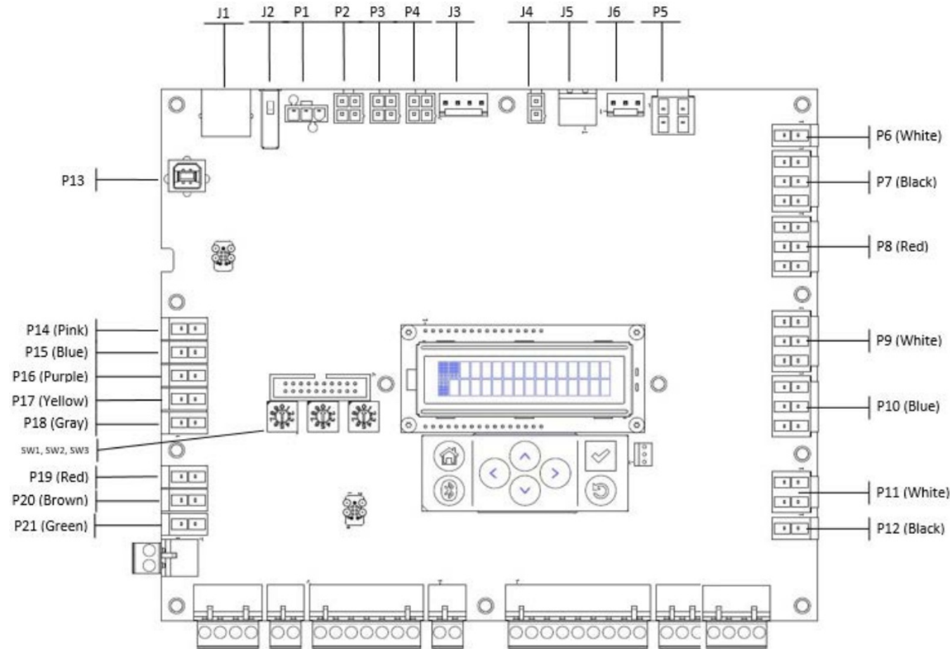
Figure 3. Symbio 700 module factory connections
