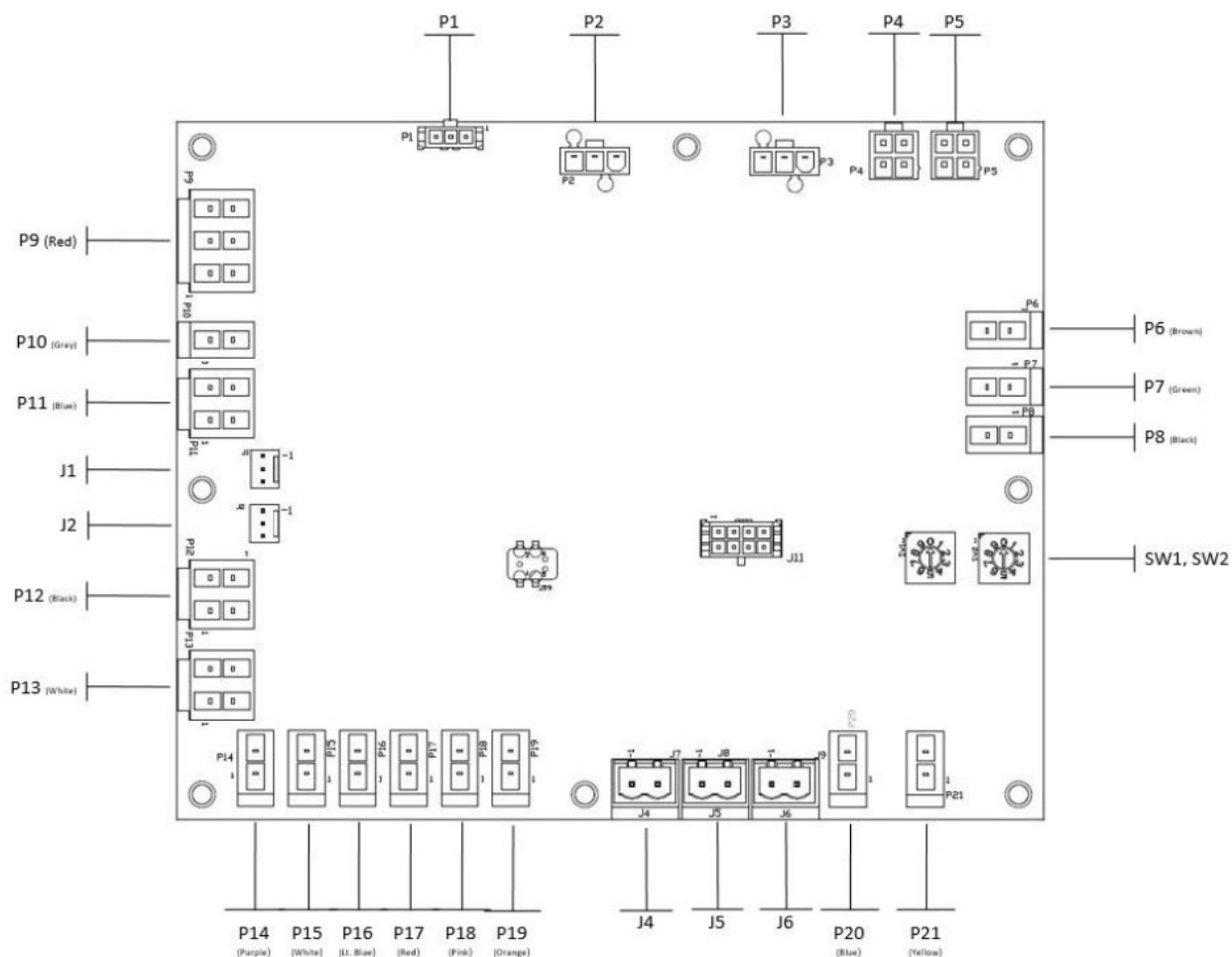
Figure 5. Symbio 700 indoor option module factory connections
