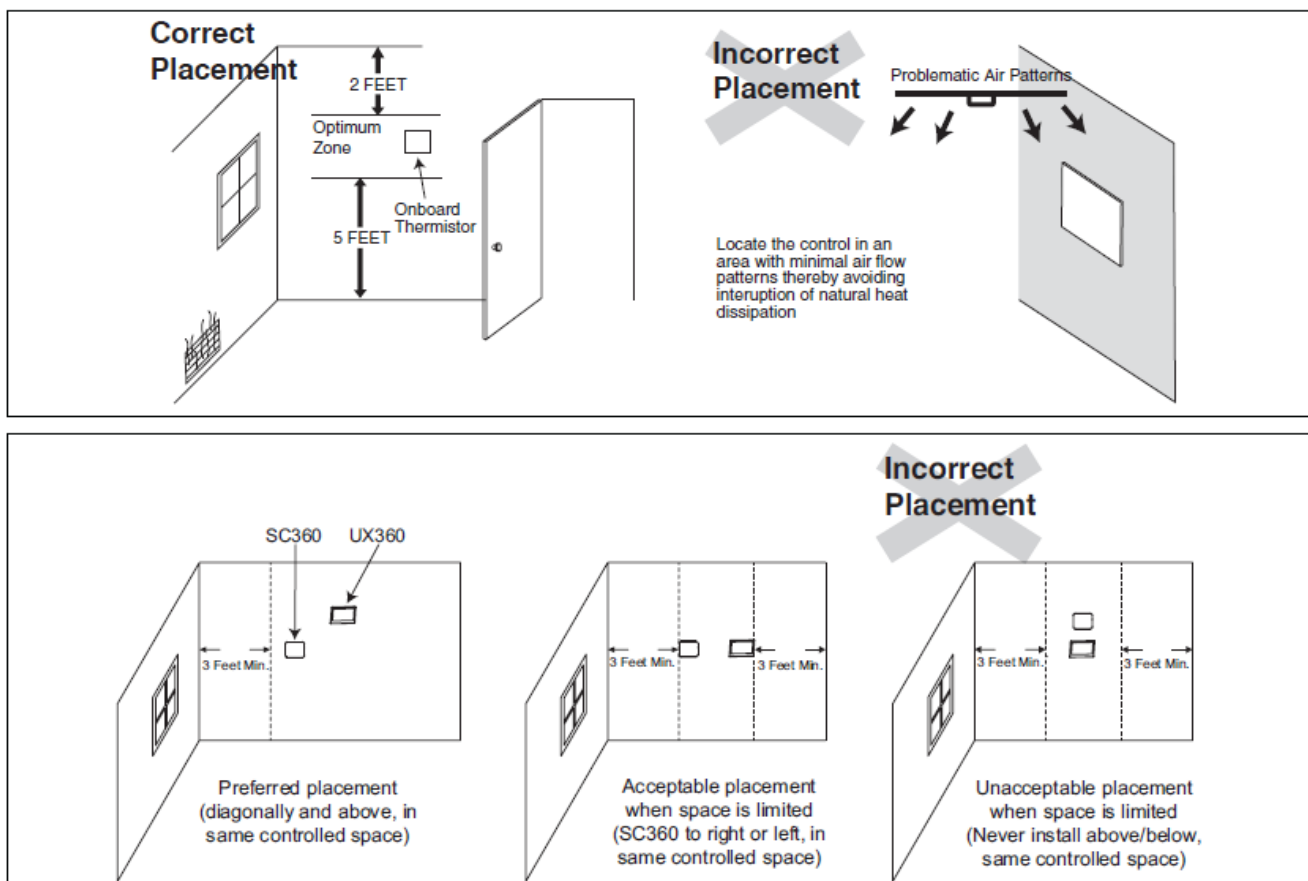
Figure 1. Placement of SC360
