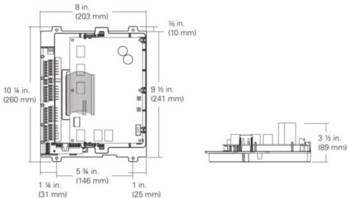
Figure 8: Frame-mounted Tracer AH541 dimensions
