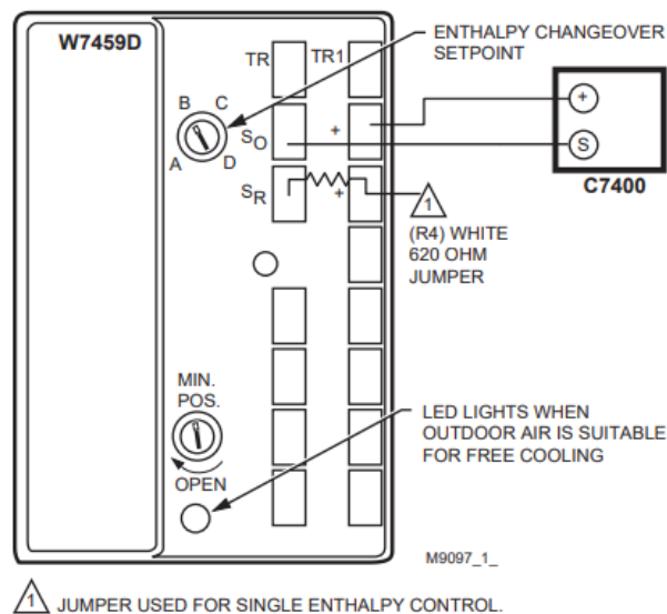
Figure 4. Control module with one enthalpy sensor
