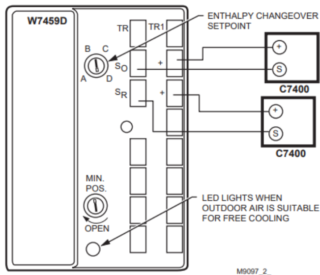
Figure 5. Control module with two enthalpy sensors
