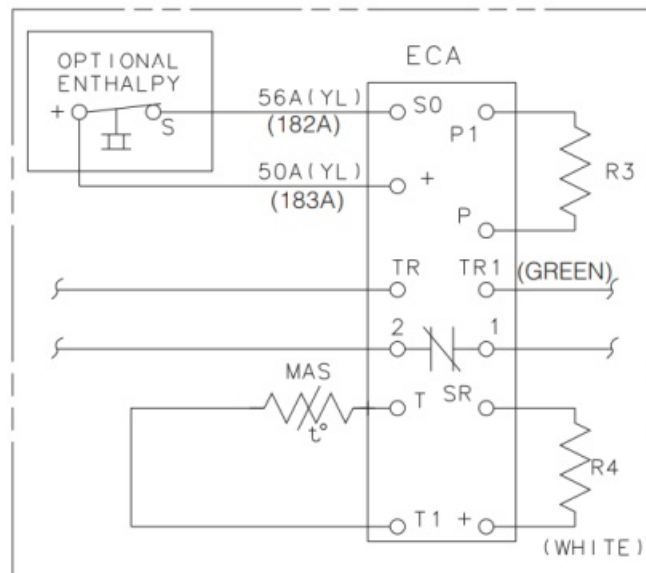
Figure 1. Enthalpy sensor wiring when used with BAYECON054, 055 & 73
