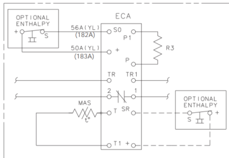
Figure 2. Economizer with optional differential enthalpy sensors
