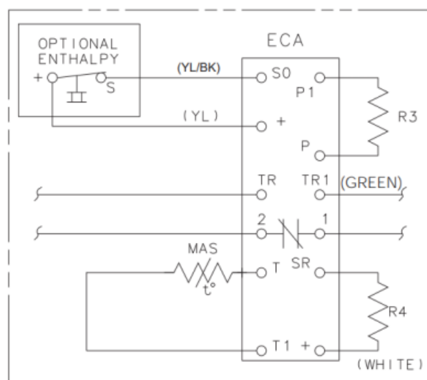
Figure 3. Economizer with optional outdoor enthalpy sensor
