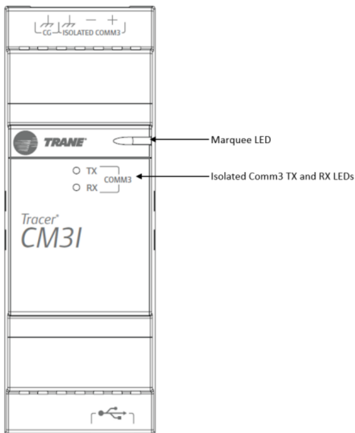
Figure 5. CM3I LEDs
