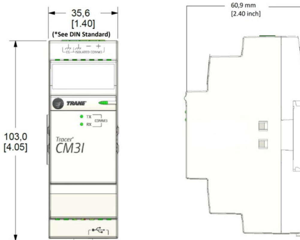
Figure 1. CM3I dimensions
