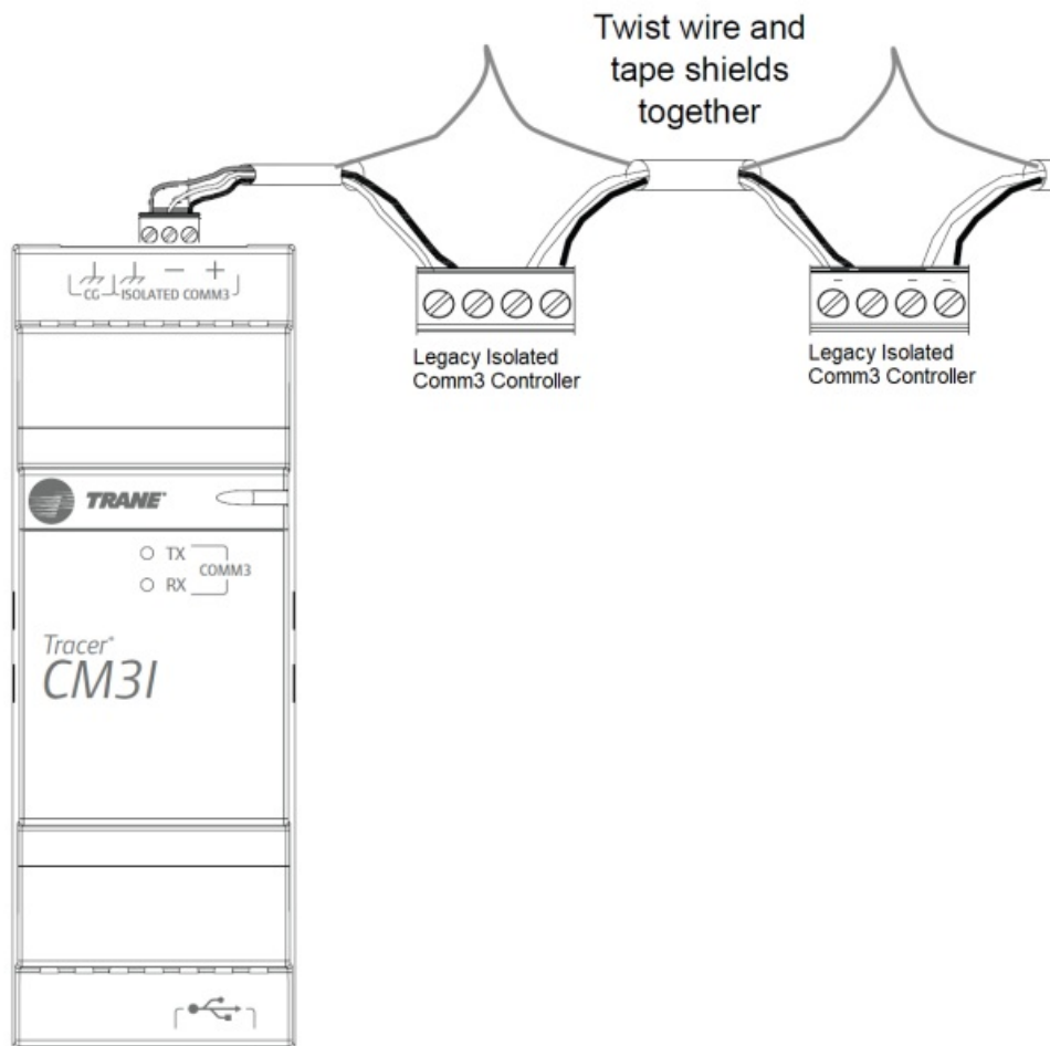
Figure 4. CM3I network wiring details
