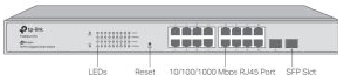
Figure 1-1 Front Panel of T1600G-18TS (TL-SG2216)
