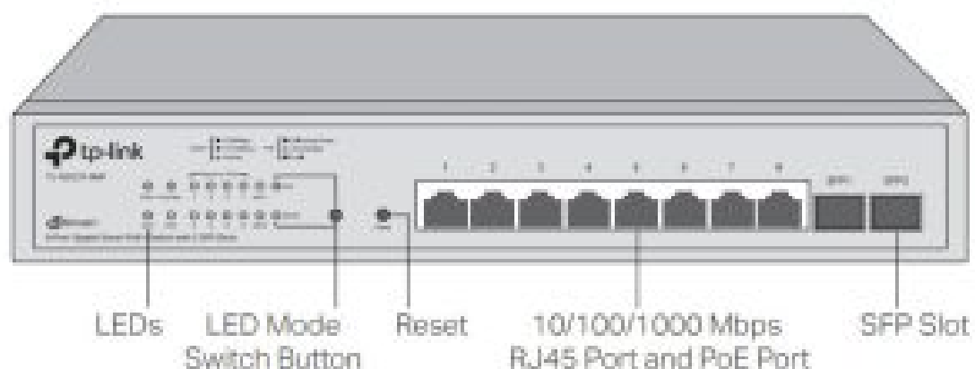
Figure 1-7 Front Panel of TL-SG2210MP
