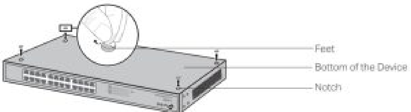
Figure 2-1 Desktop Installation
