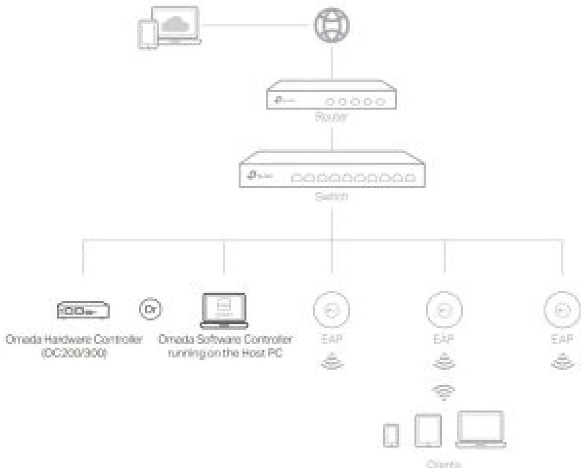
Figure 4-2 Manage the network via Omada Software/Hardware Controller
