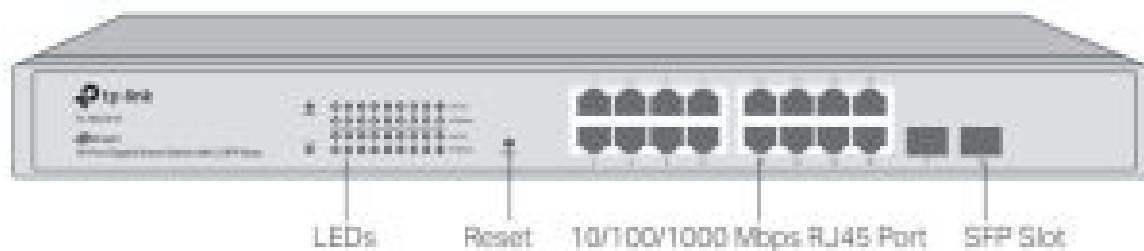
Figure 1-6 Front Panel of TL-SG2218
