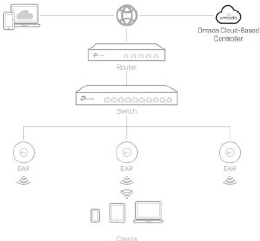
Figure 4-3 Manage the network via Omada Cloud-Based Controller
