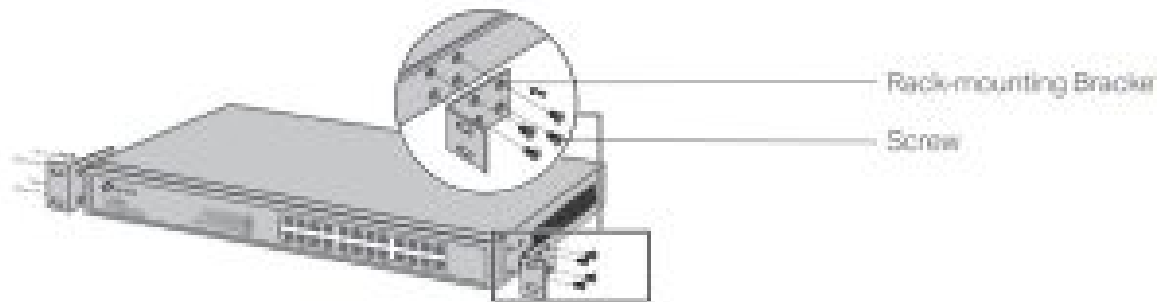
Figure 2-2 Bracket Installation
