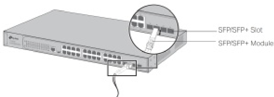
Figure 3-2 Inserting the SFP Module
