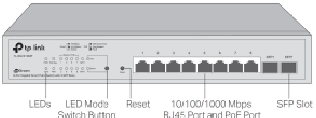
Figure 1-7 Front Panel of TL-SG2210MP
