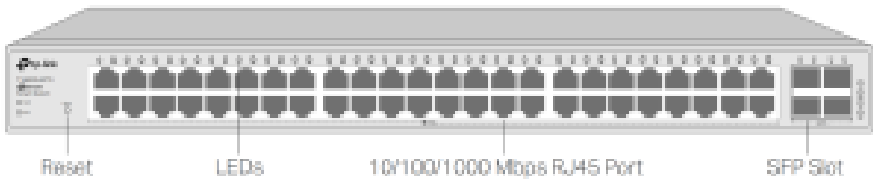
Figure 1-2 Front Panel of T1600G-52TS (TL-SG2452)
