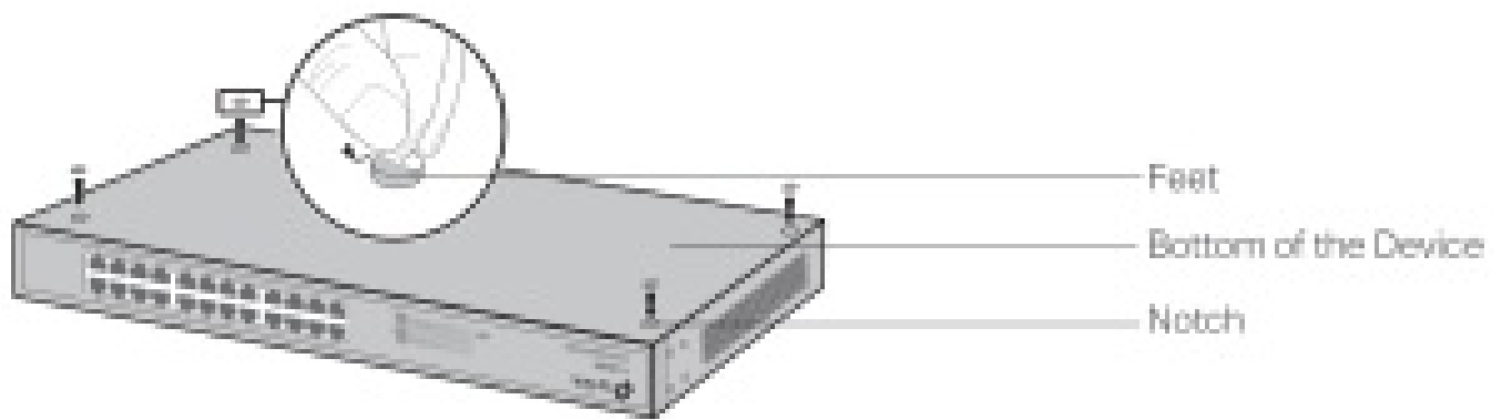
Figure 2-1 Desktop Installation
