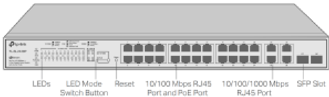
Figure 1-9 Front Panel of TL-SL2428P
