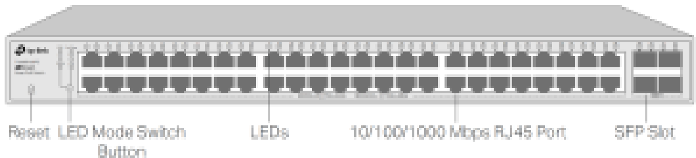
Figure 1-3 Front Panel of T1600G-52PS (TL-SG2452P)
