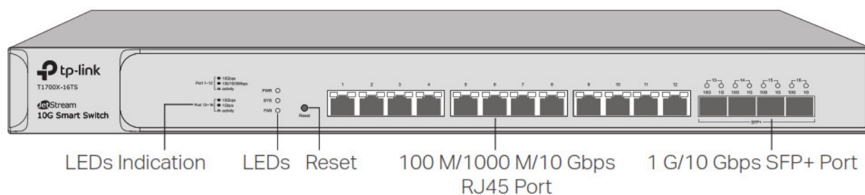
Front Panel of T1700X-16TS
