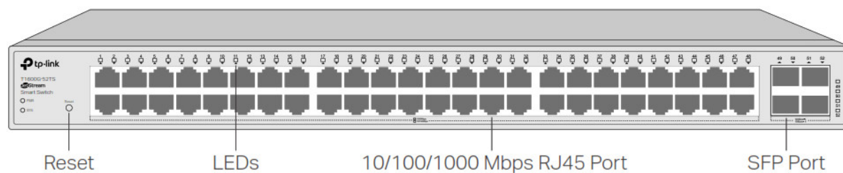
Front Panel of T1600G-52TS (TL-SG2452)
