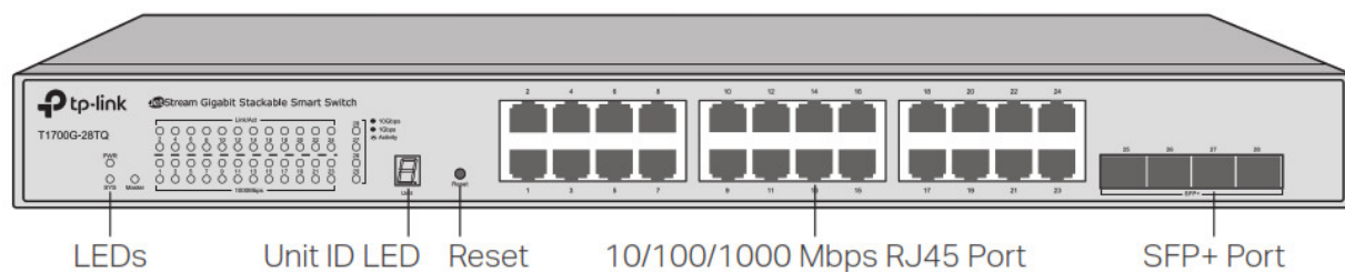
Front Panel of T1700G-28TQ
