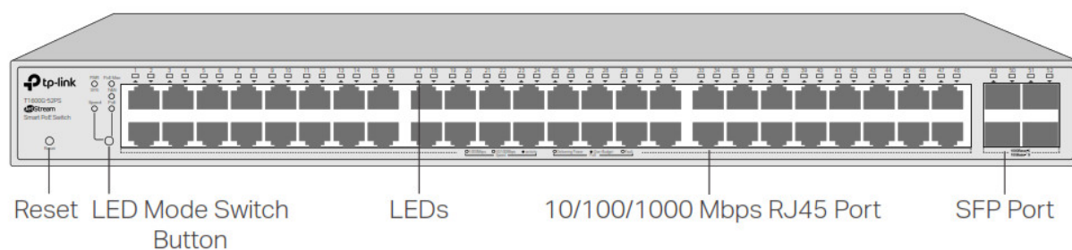
Front Panel of T1600G-52PS (TL-SG2452P)
