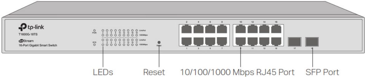
Figure 1-2 Front Panel of T1600G-18TS (TL-SG2216)
