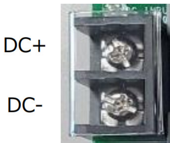
Fig. 4.2 Motor Power Input Connector on Board (J1)
