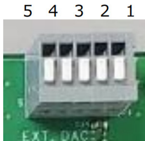
Fig. 4-9 External DAC Connector (J4)
