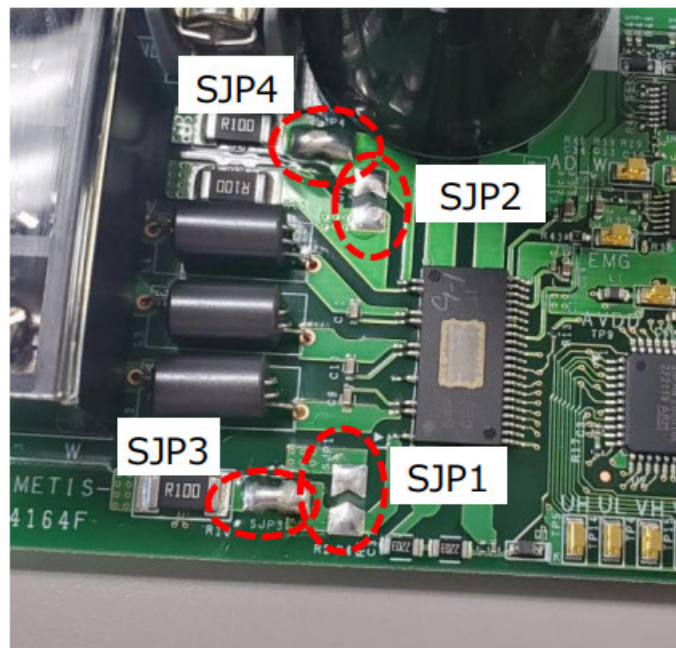
Fig. 4.1 Solder Jumpers on the Board
