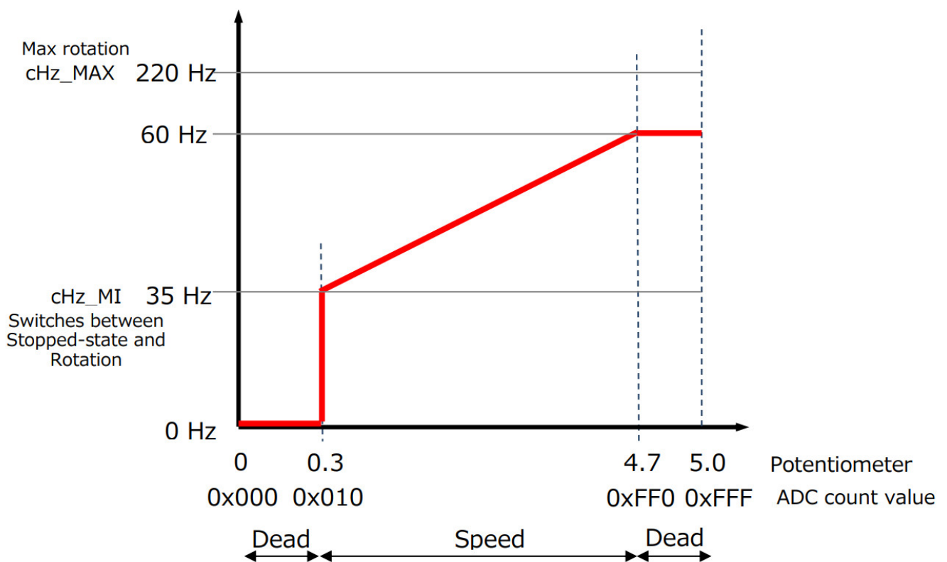
Fig. 4.7 Relationship between potentiometer setting value and rotational speed
