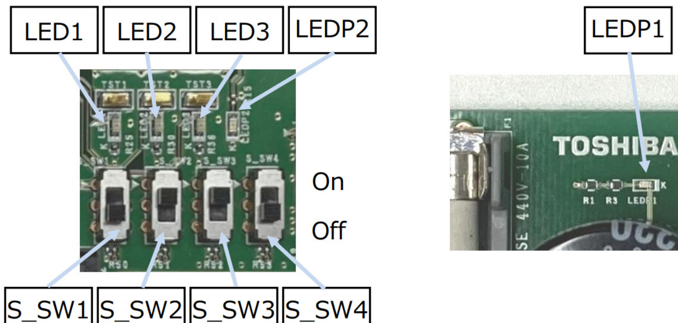
Fig. 4.5 Switches and LEDs on the Board
