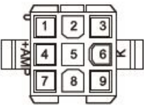
AMP 172332-1 BACK VIEW
