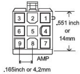
AMP 172340-1 BACK VIEW
