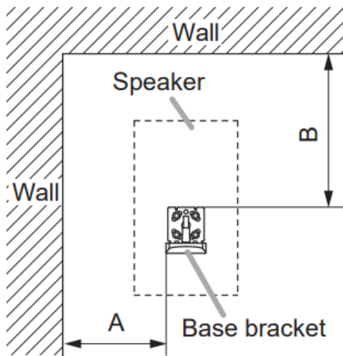
(Vertical installation)
