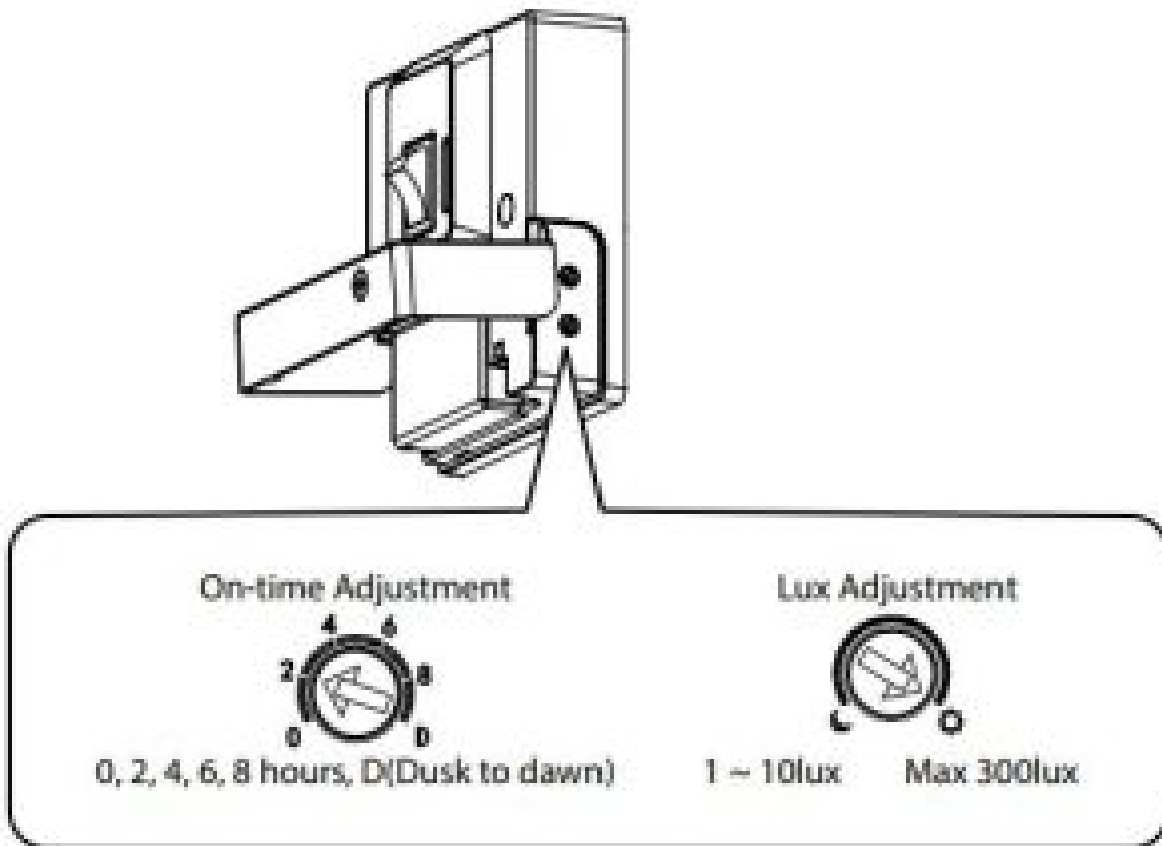
Fig 7 – On-time and Lux Adjustment
