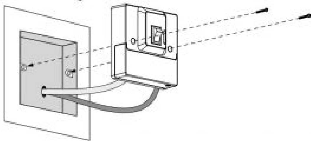
Fig 5 – Installation
