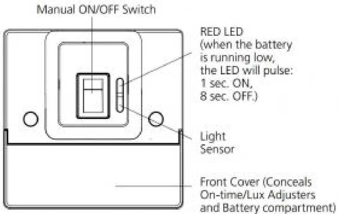
Fig 1 – Front Face
