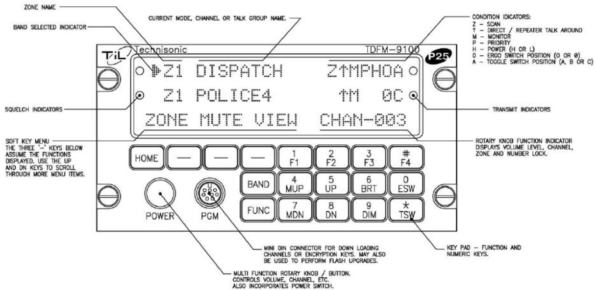
FIGURE 1: Front Panel Controls – TDFM-9100 Transceiver
