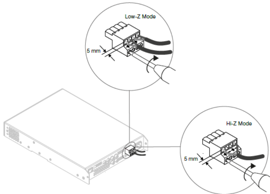
Diagram 6d GPIO cable connections. 5 mm
