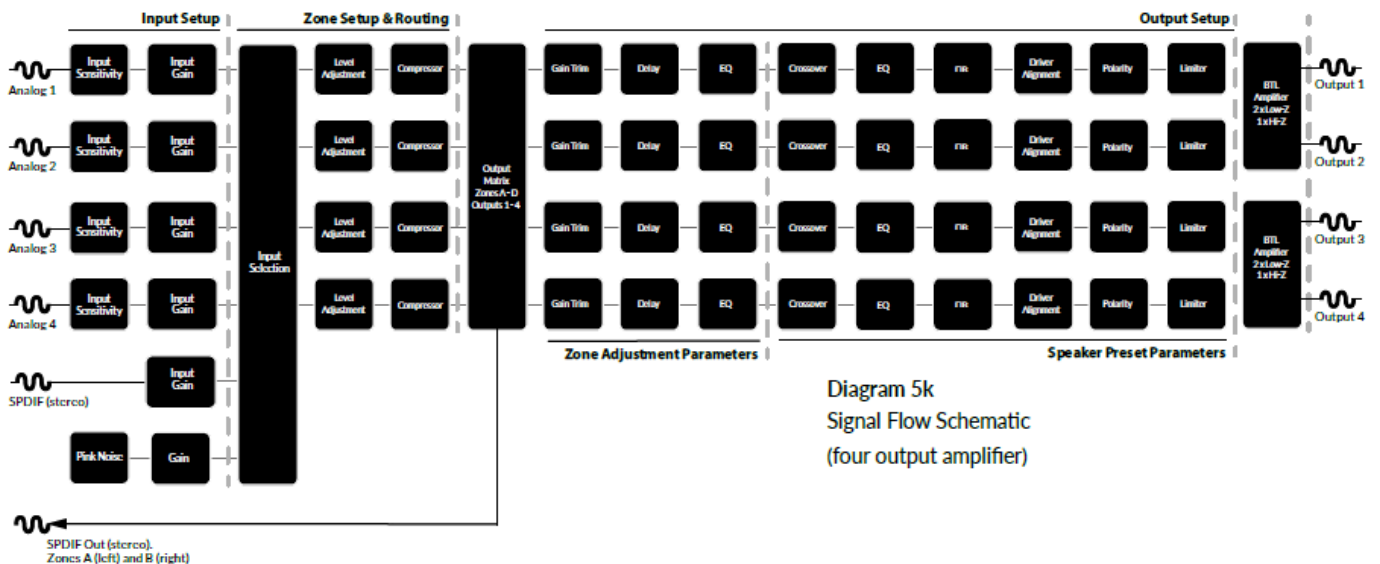
Diagram 5k Signal Flow Schematic (four output amplifier)
