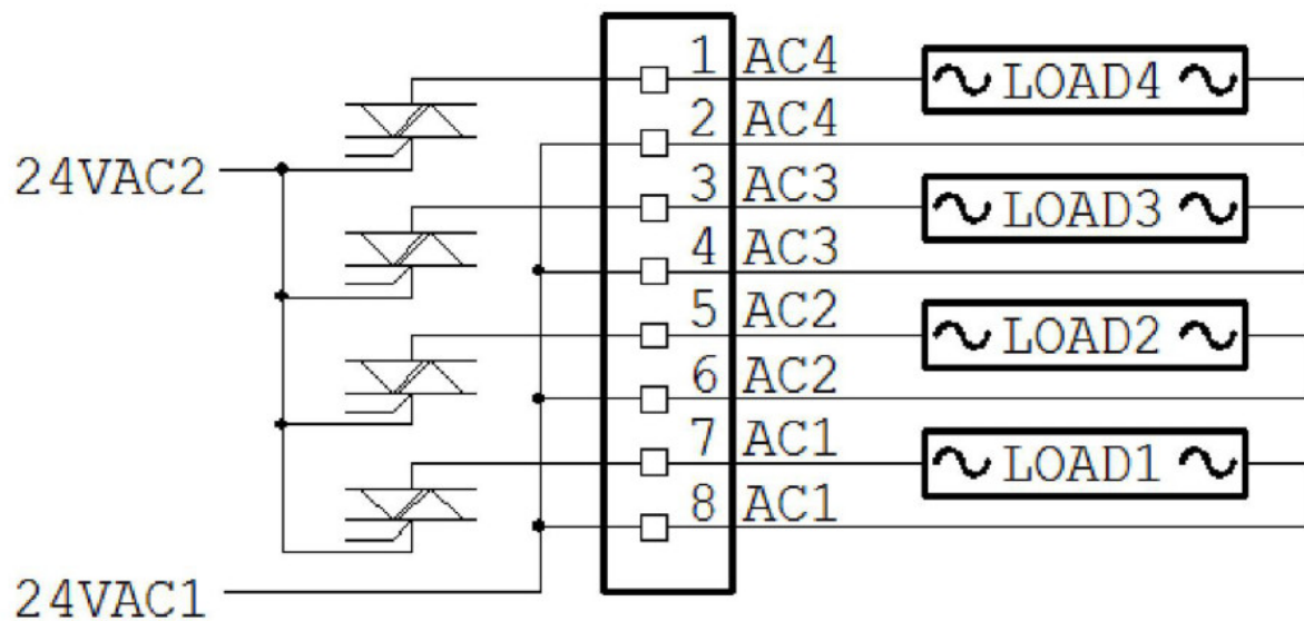
TRIAC OUTPUTS CONFIGURATION. MAX LOAD = 1A
