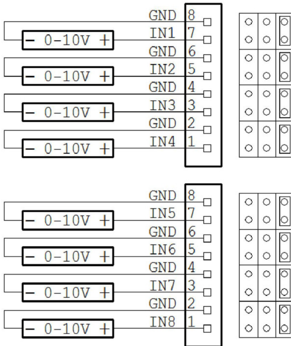
0-10V INPUTS CONFIGURATION
