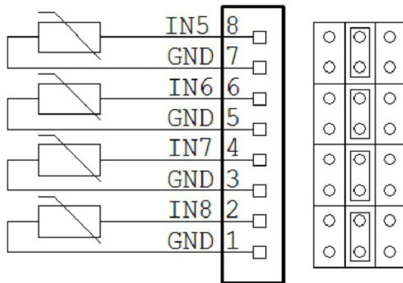
TEMPERATURE MEASUREMENT CONFIGURATION WITH 1K THERMISTORS
