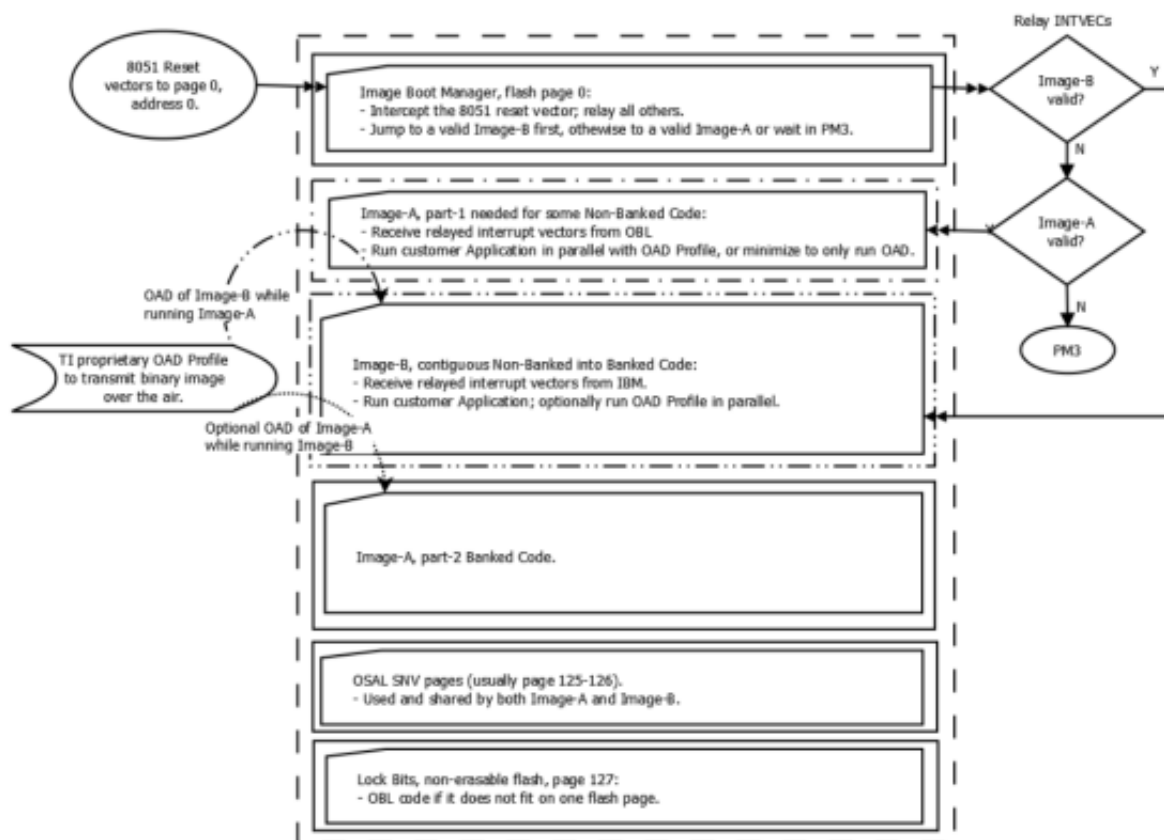
Figure 2: OAD Target Context Diagram using a BIM.
