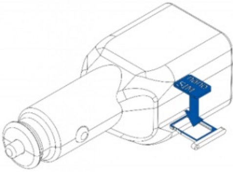
Figure 3 Nano-SIM card insert
