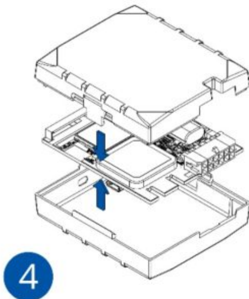
4. Figure 7 Attaching cover back
