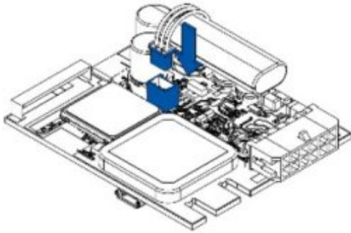
3. Figure 5 Battery connection
