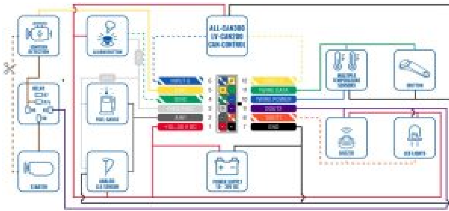
Figure 3 FMB120 Wiring scheme
