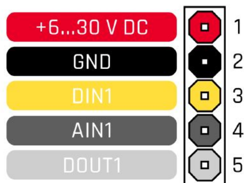
Figure 2 FMB920 pinout
