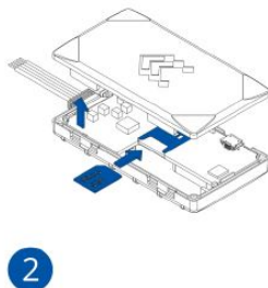
Figure 5 Micro-SIM card insert
