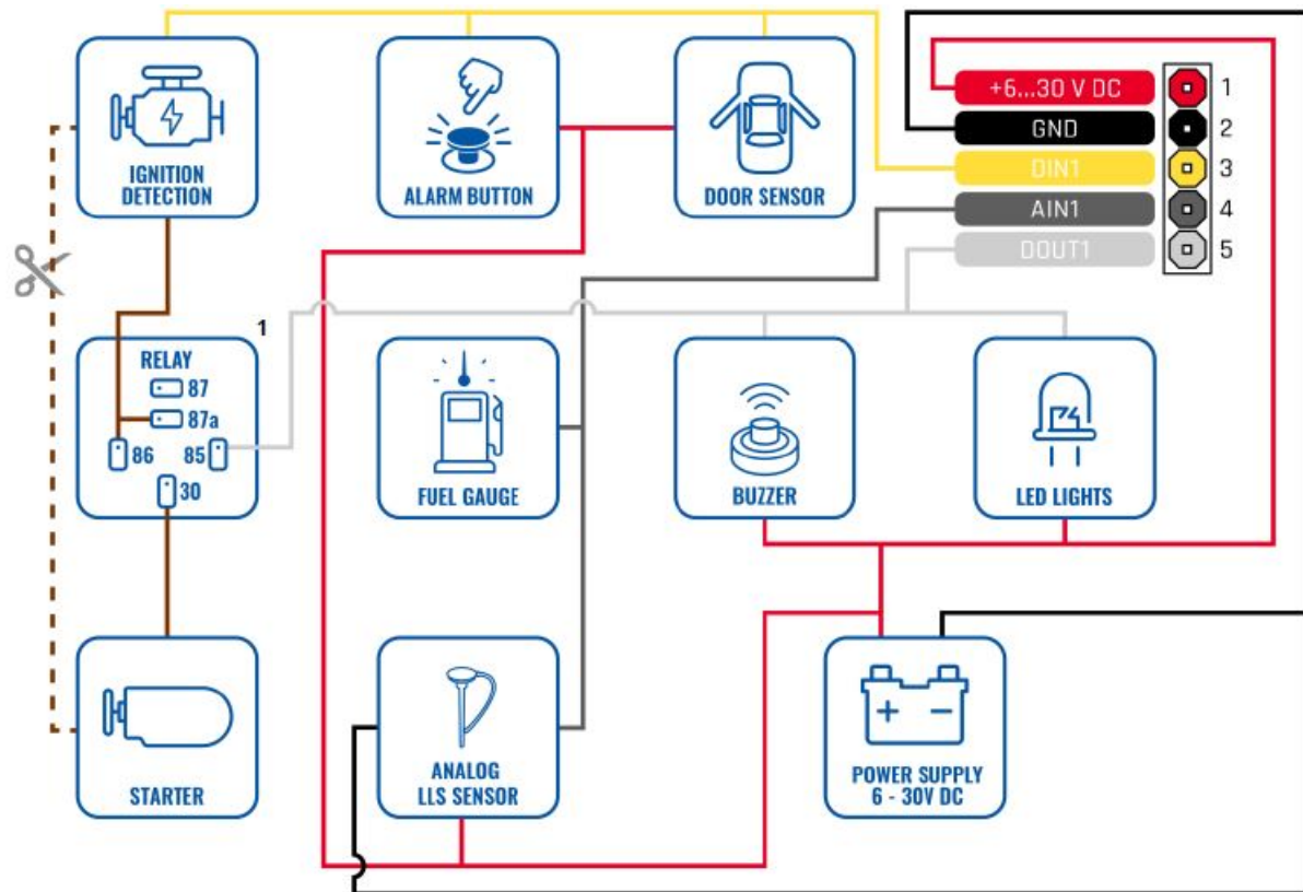
Figure 3 FMB920 Wiring scheme
