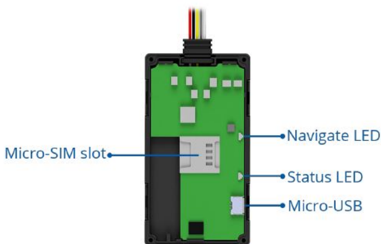
Figure 1 FMB920 device view
