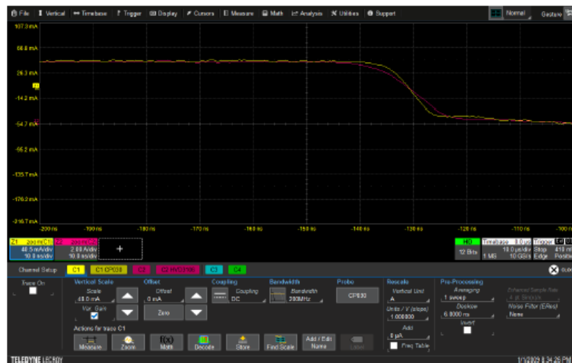
Voltage and current waveforms following deskew.
