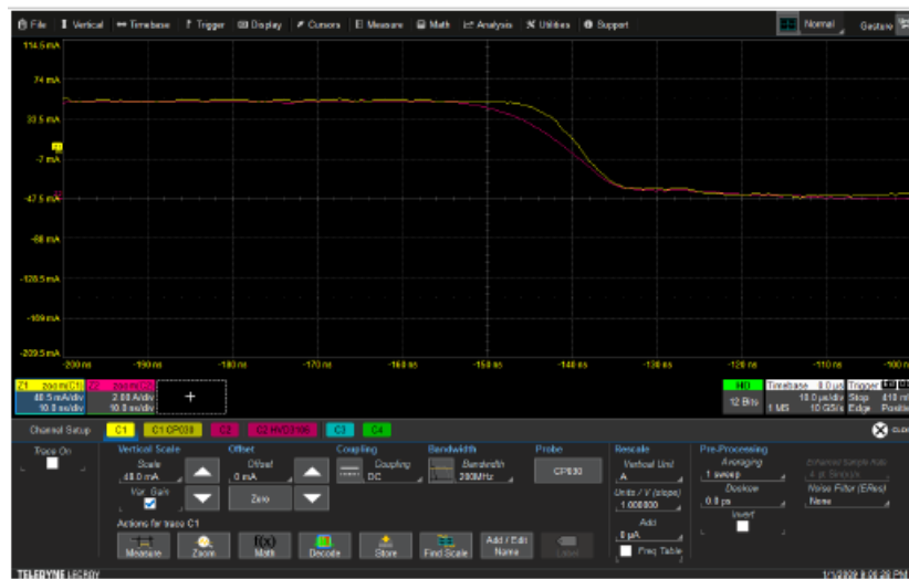
Voltage and current waveforms prior to deskew.
