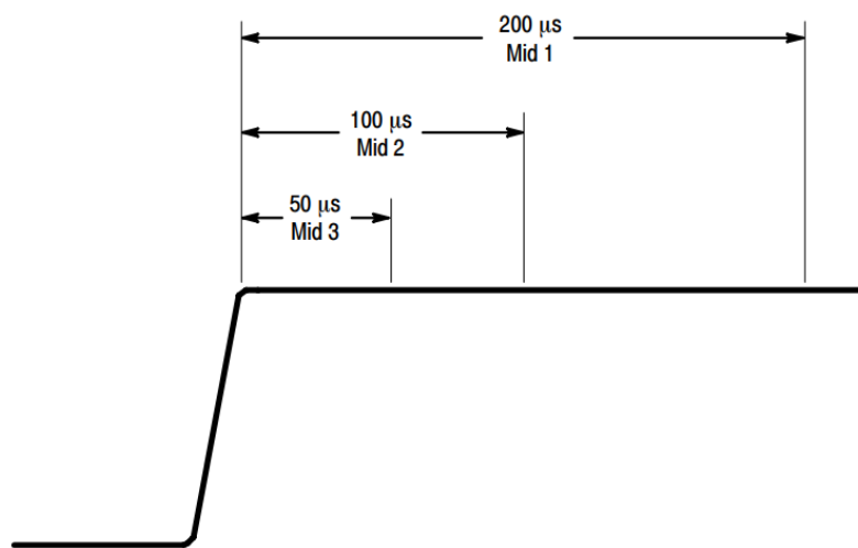
Figure 1-6: Zones Affected by Compensation Adjustments
