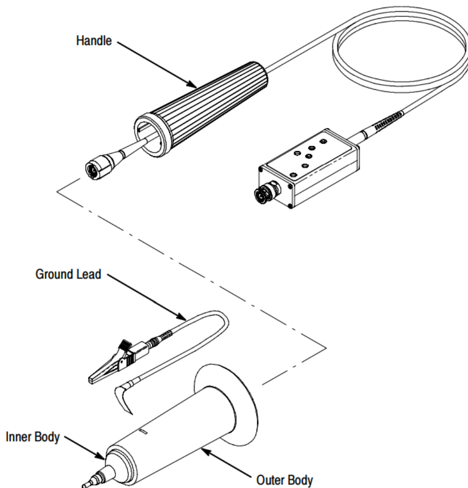
Figure 1-3: Assembling the P6015A
