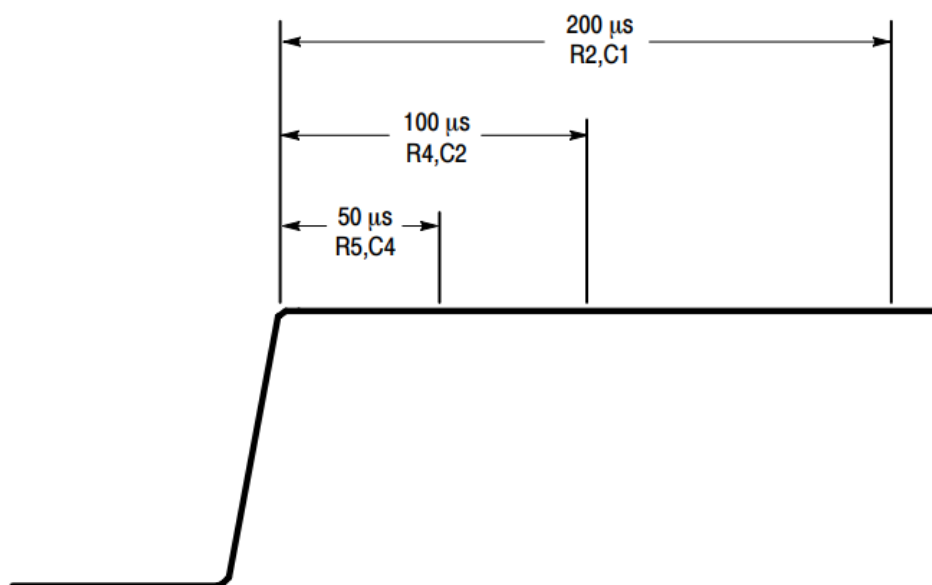
Figure 2-3: Periods Affected by Compensation Adjustments
