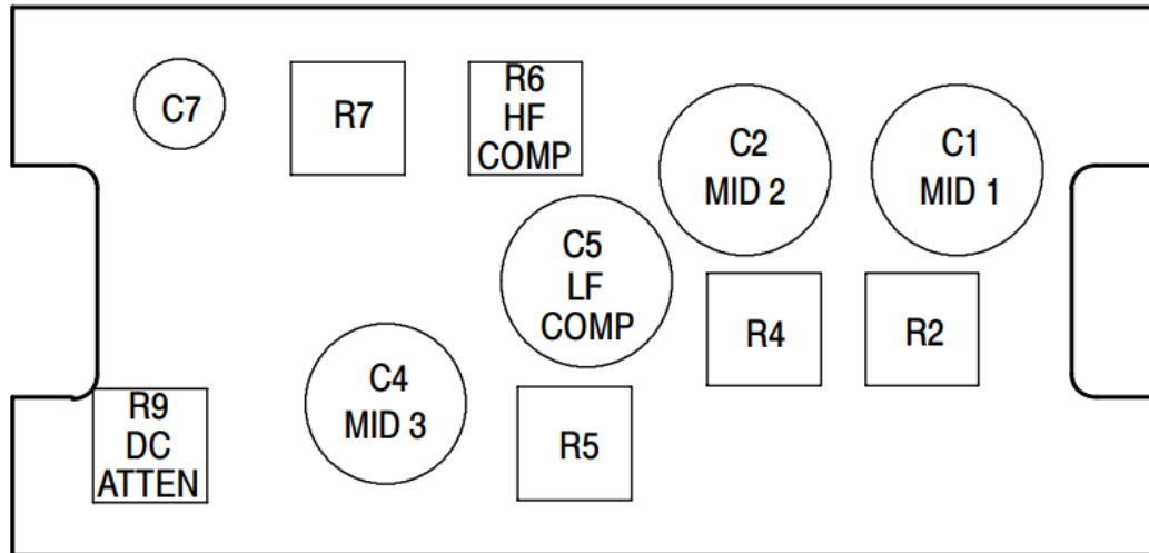
Figure 2-2: Adjustment Locations
