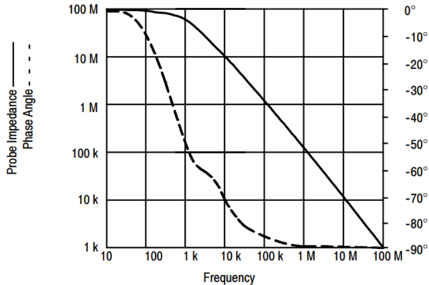
Figure 1-8: Typical Input Impedance and Phase
