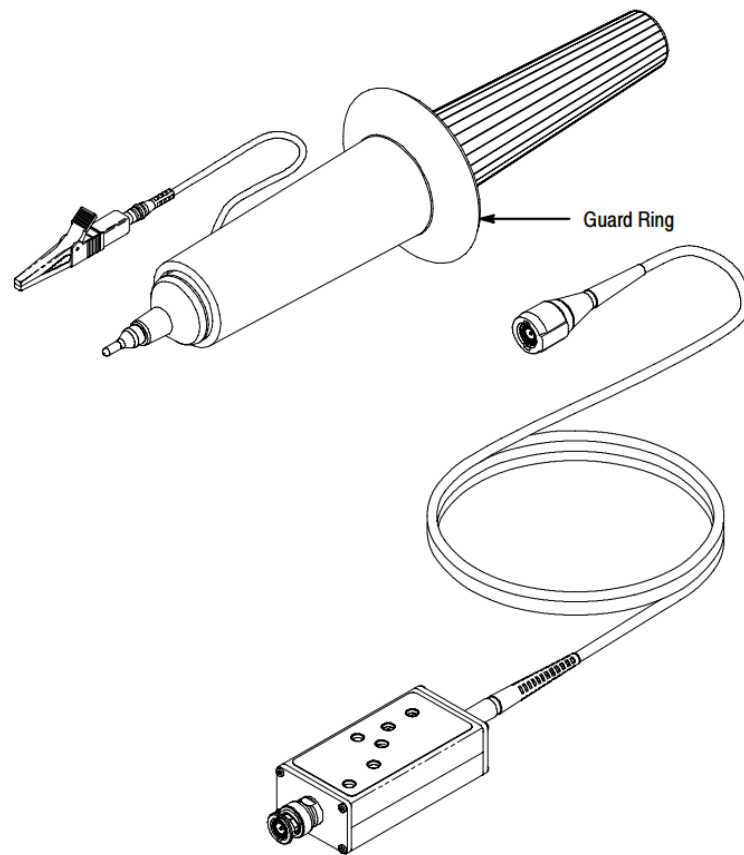
Figure 1-1: The P6015A High-Voltage Probe
