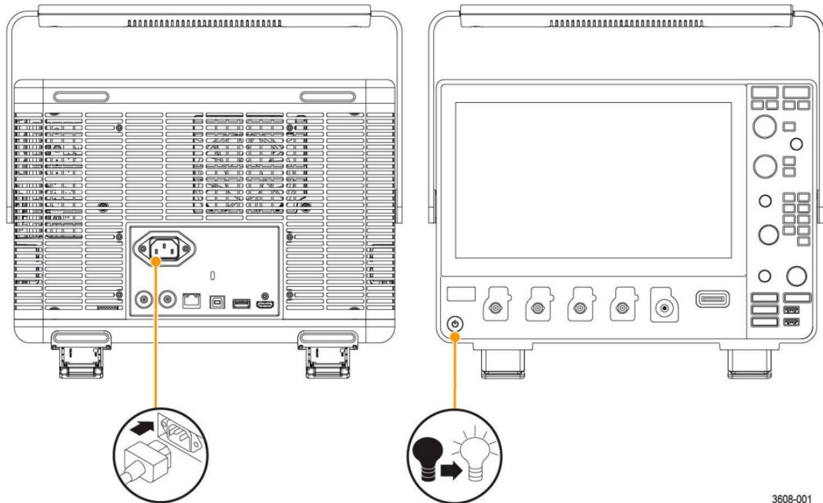
Figure 1: Power cord connector and power standby switch
