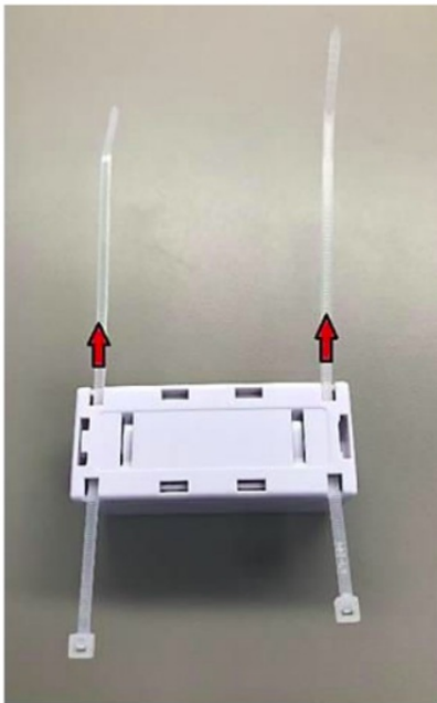
Figure 2-3: Threading Zip Ties Through the Mounting Holes to Fasten the Tracker
