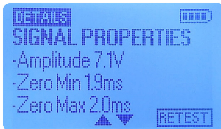
Figure 3: IRIG-B Analyzer Signal Properties
