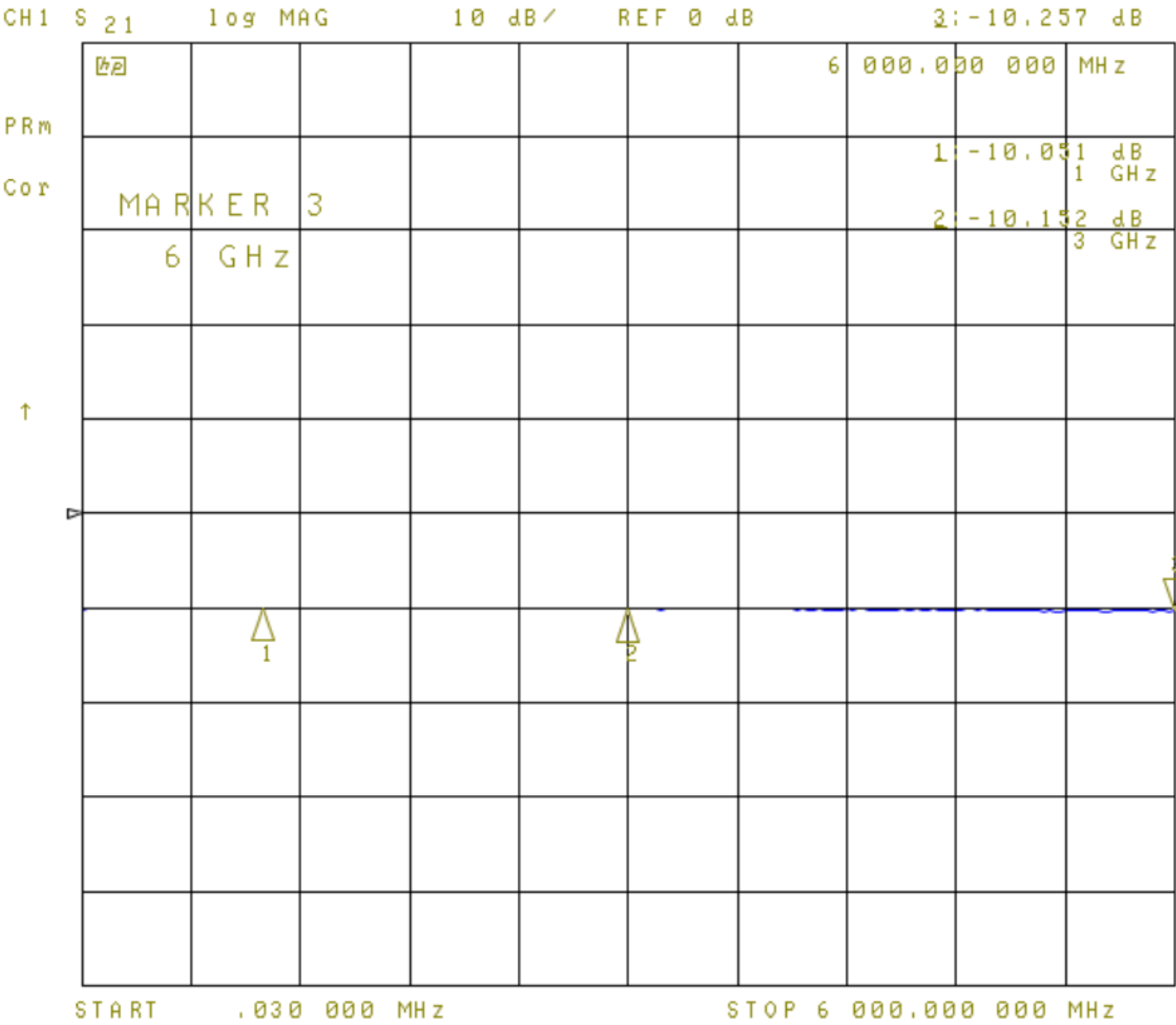
10dB Attenuator, S21
