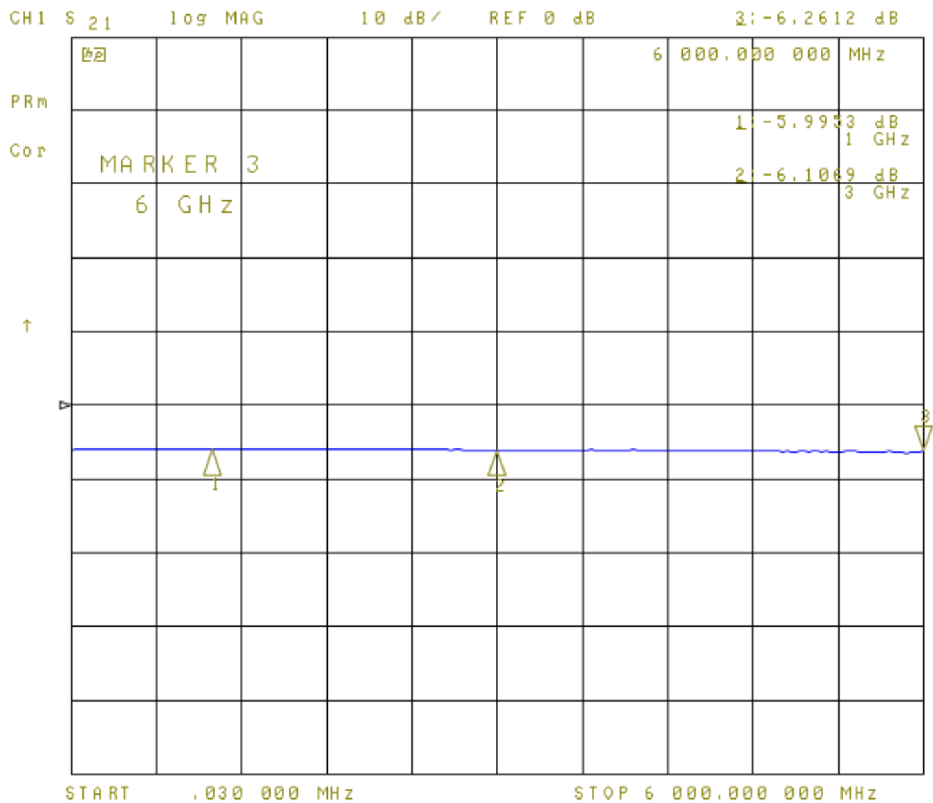
6dB Attenuator, S 21
