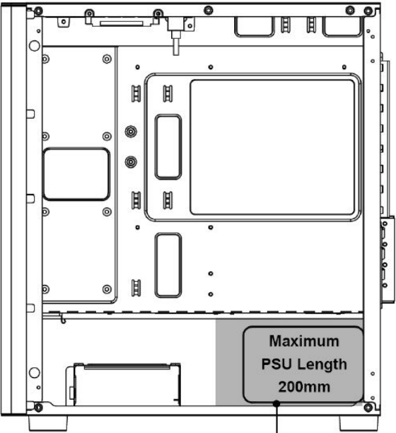
Power Supply Unit Installation
