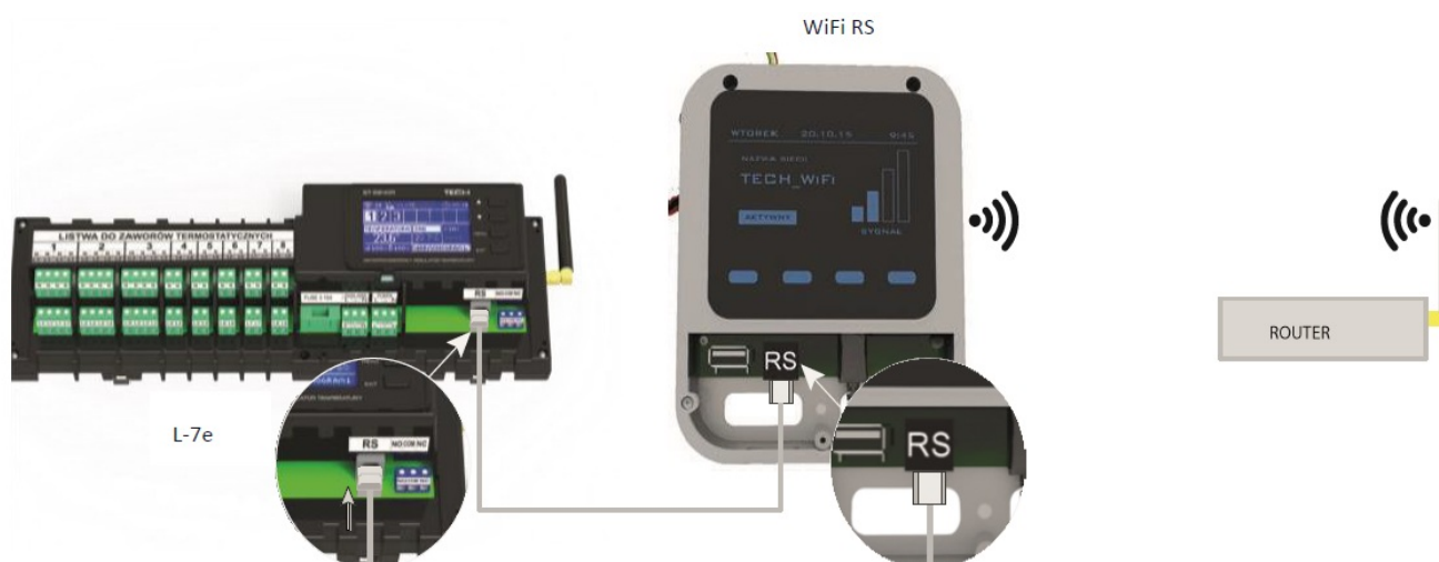
Connection diagram for WiFi RS Internet module.
