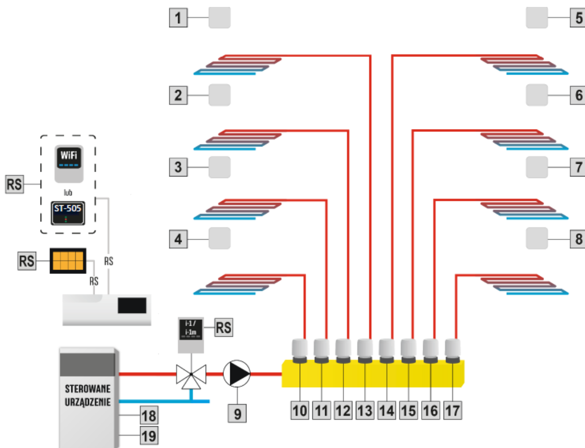
Pictorial diagram presenting wiring and communication with other devices in the system:
