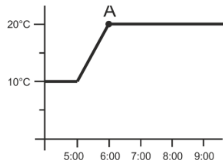
Room temperature - OPTIMUM START ON
