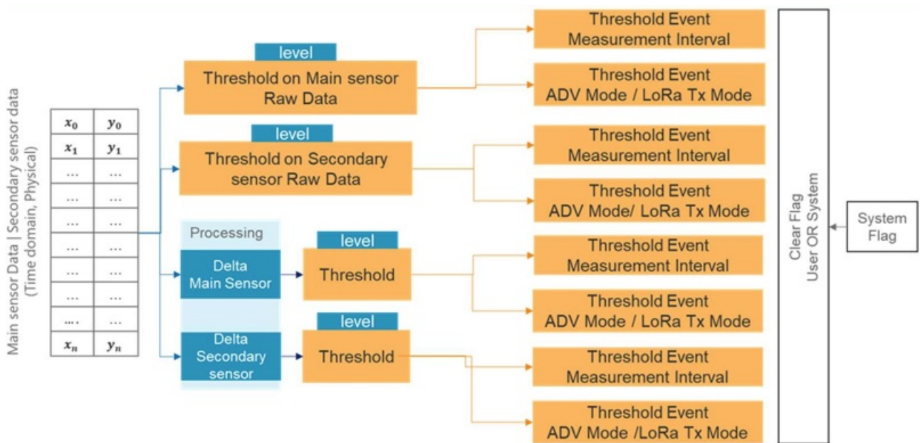
Threshold manager bloc diagram
