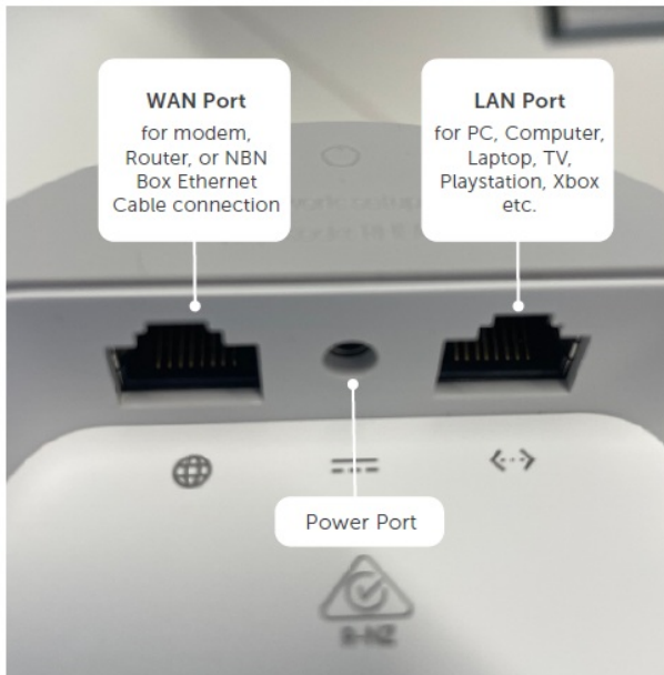
Router underneath view
