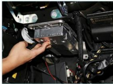
TAKE OUT PLUG OF CONTROL BOX BEHIND HAND GLOVE COMPARTMENT
