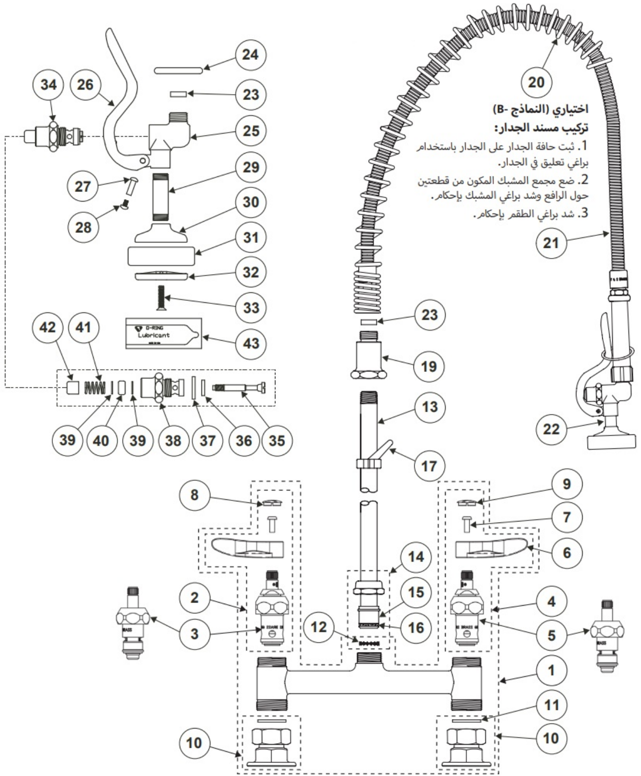
Base Faucet Assemblies
